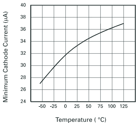
Izmin vs. Temperature
