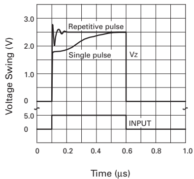
Pulse Response
