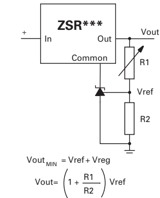
Output control of a three terminal fixed regulator
