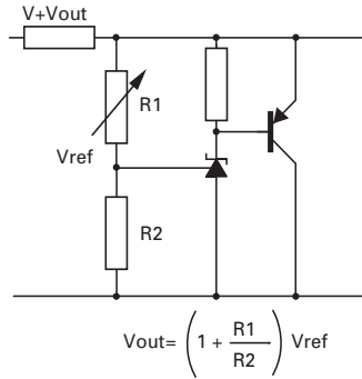
Higher current shunt regulator
