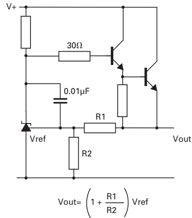
Series regulator
