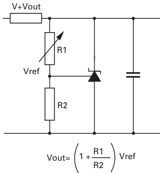
Shunt regulator
