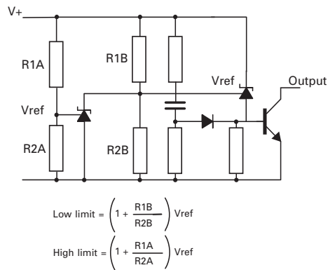
Over voltage / under voltage protection circuit
