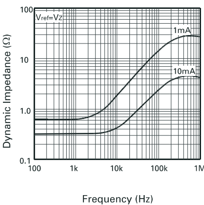
Dynamic Impedance v Frequency
