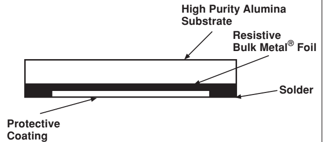
FIGURE 3 - CHIP CONFIGURATION
