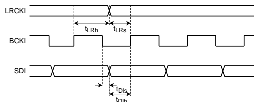
Figure 7.3 Digital Data Input/Output Timing
