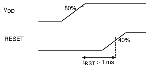
Figure 6.2 Power-On Reset Timing
