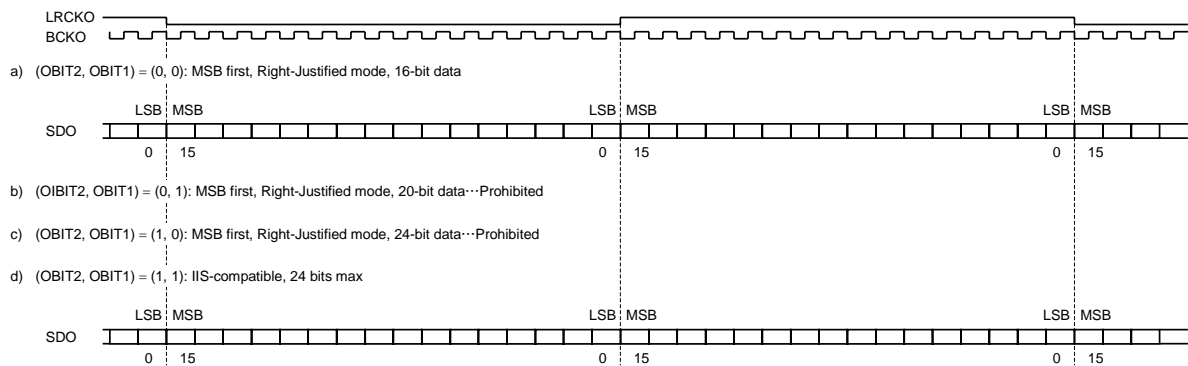
Figure 2.2 Data Output Formats
