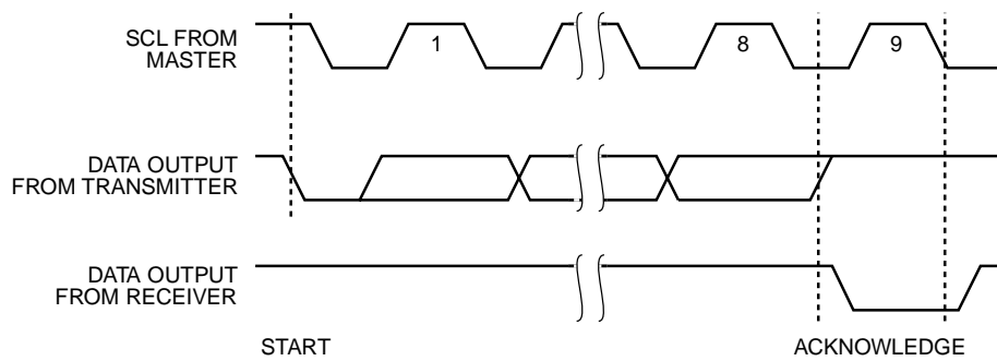
Figure 3. Acknowledge Timing
