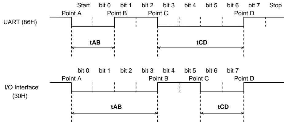
Figure 3.2 Serial Operation Mode Byte
