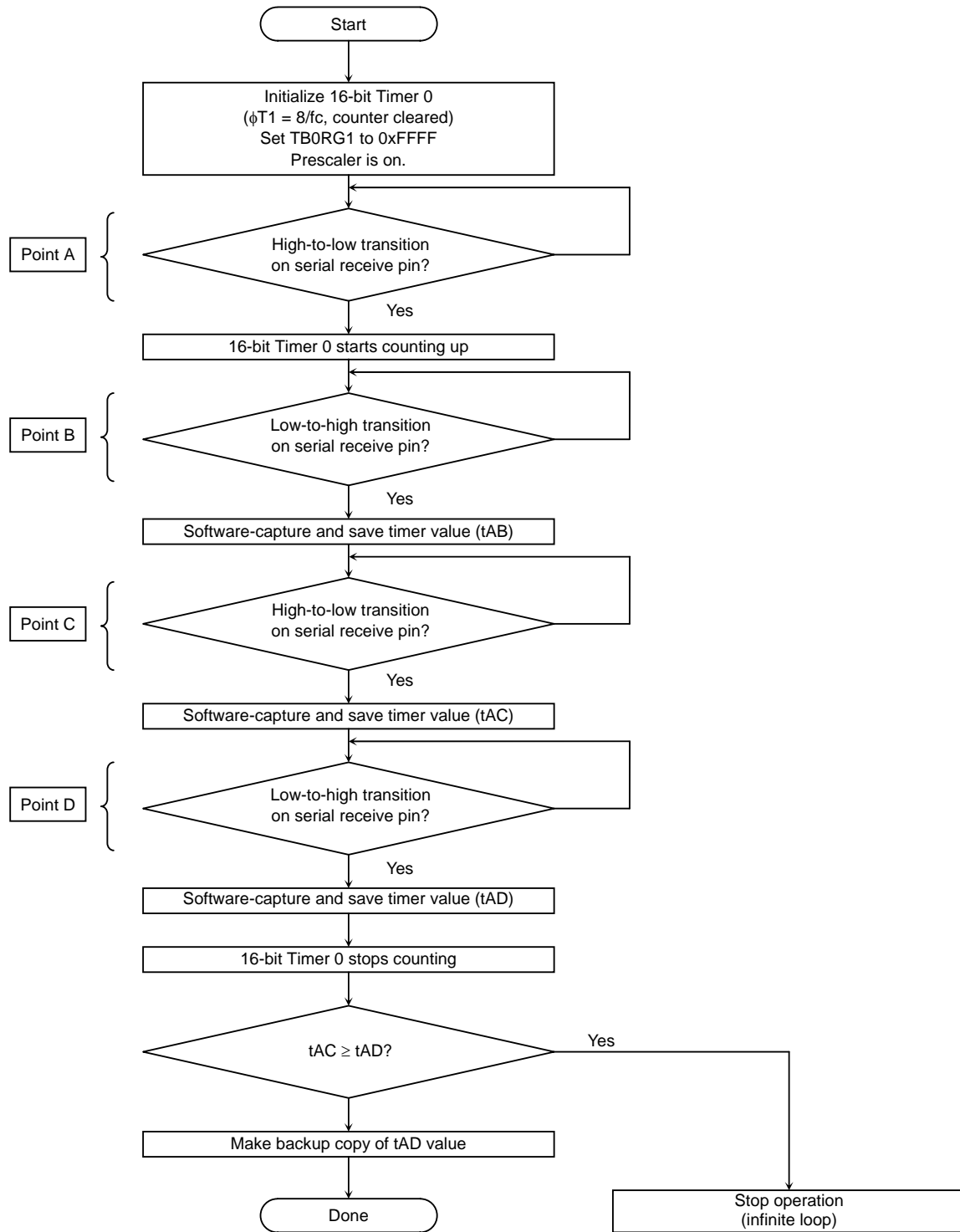
Figure 3.3 Serial Operation Mode Byte Reception Flow
