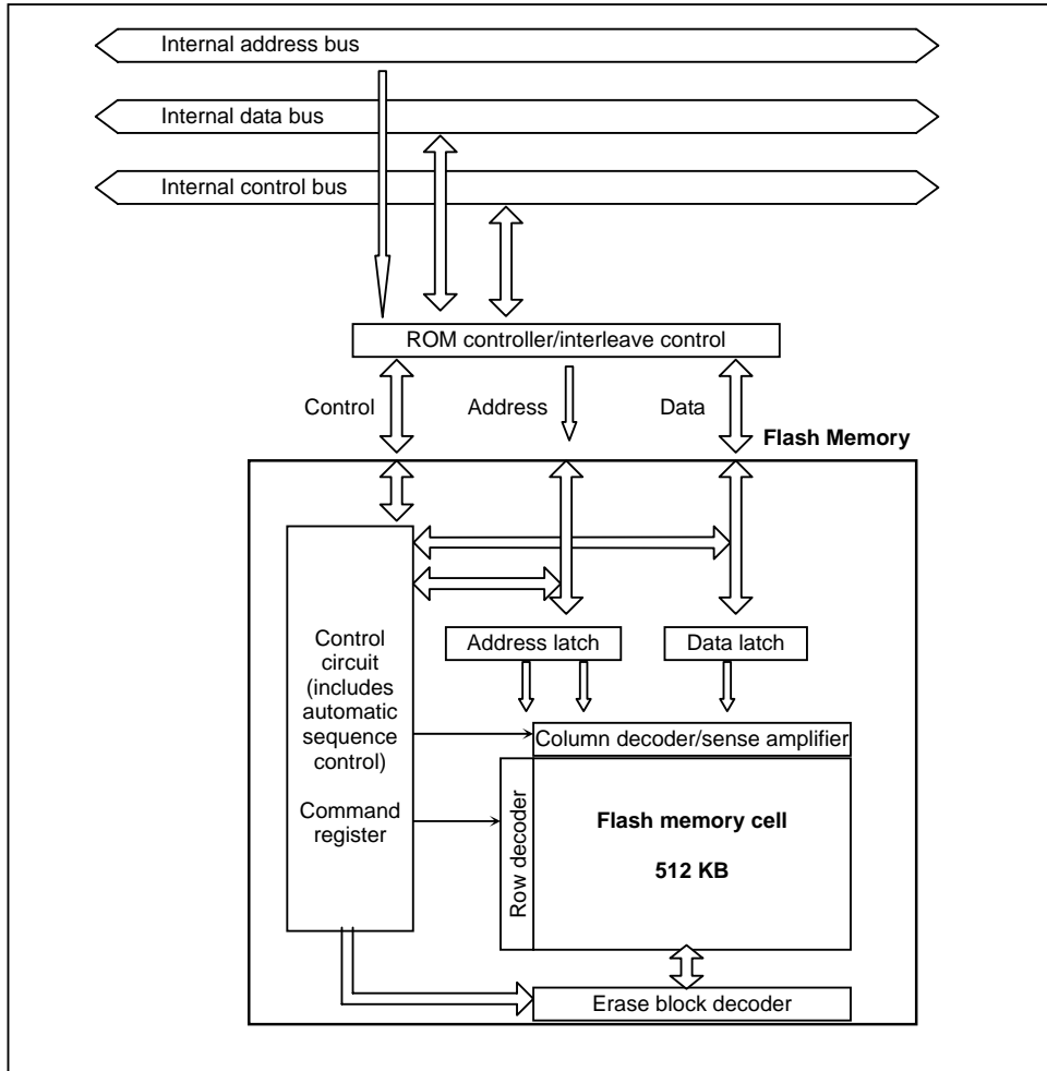
Fig. 3-1 Block Diagram of the Flash Memory Section
