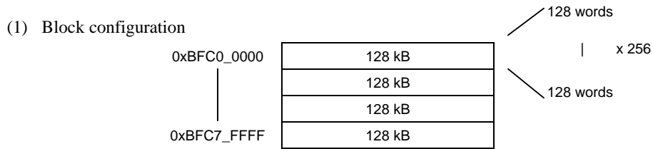
Fig. 3-4 Block Configuration of Flash Memory
