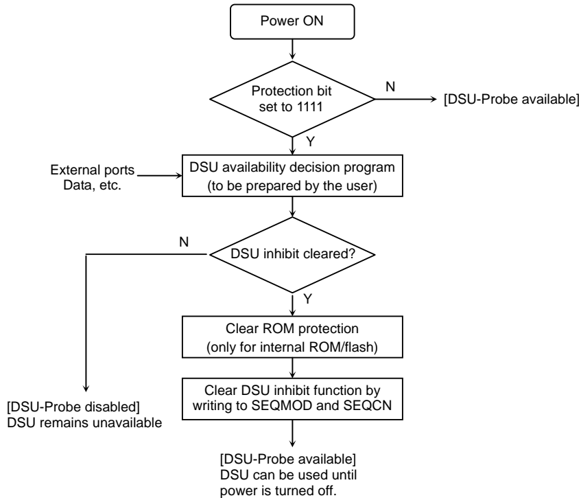
Figure 3-3 Example Use of DSU Inhibit Function
