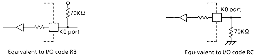
Figure 1-2. I/O code and external circuitry
