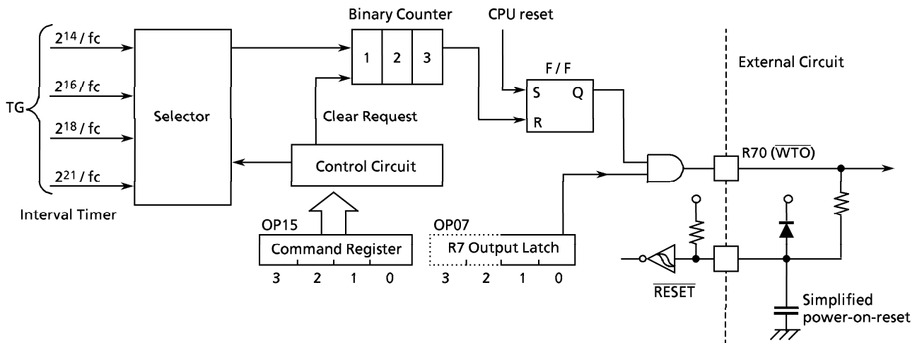
Figure 3-14. Watchdog Timer
