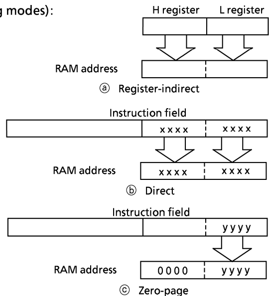
Figure 2-5. Addressing mode
