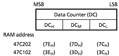
Figure 2-7. Data Counter
