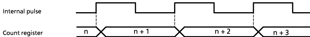
Figure 3-12. Timer Mode Timing chart
