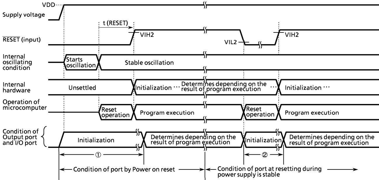
Figure 3-16. Port condition by Reset operation
