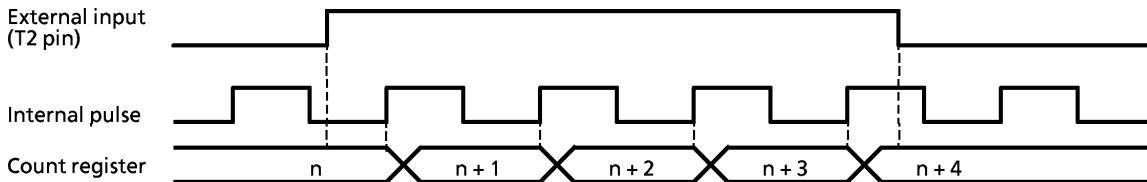
Figure 3-13. Pulse Width Measurement Mode Timing chart
