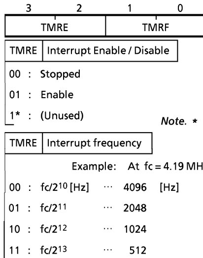
Figure 3-7. Command Register
