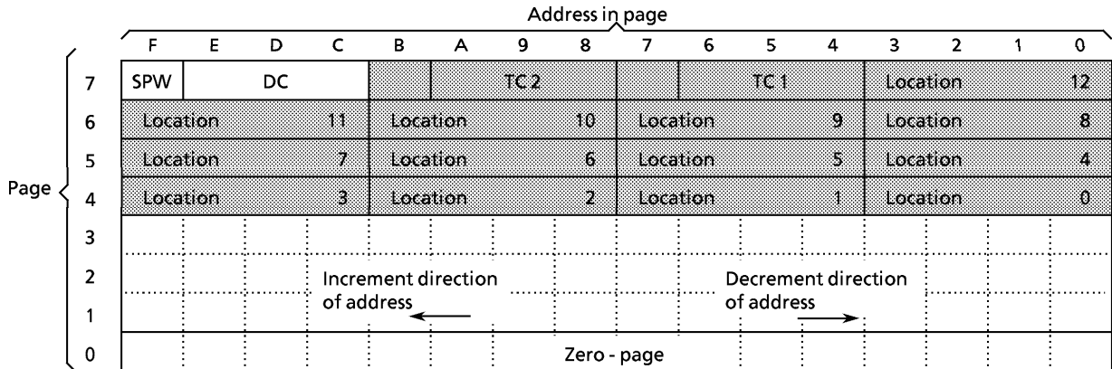
Figure 2-6. Data Memory Map (47C202)
