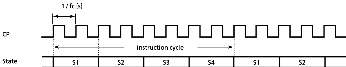
Figure 2-17. Instruction Cycle
