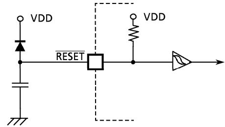
Figure 2-23. Simplified Power-On-Reset
