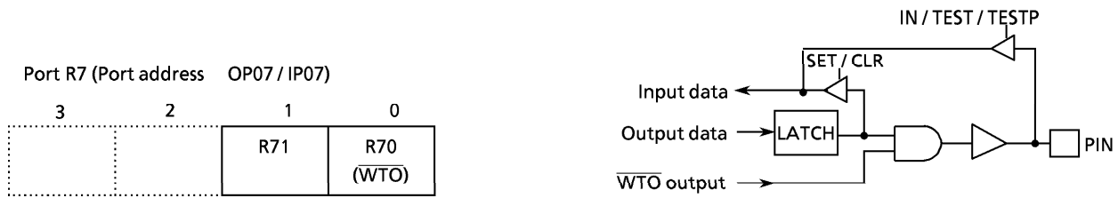
Figure 3-4. Ports R7
