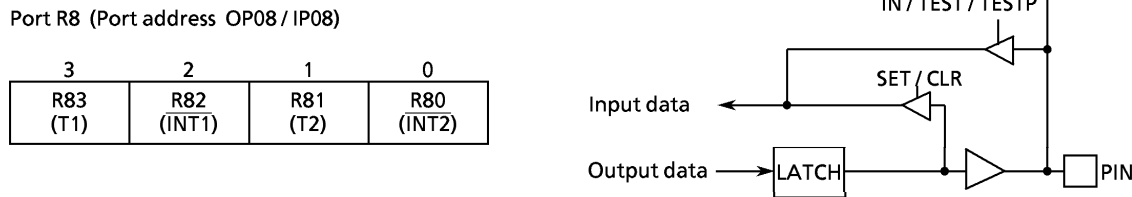
Figure 3-5. Port R8
