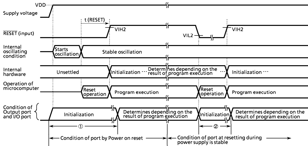
Figure 3-12. Port condition by Reset operation
