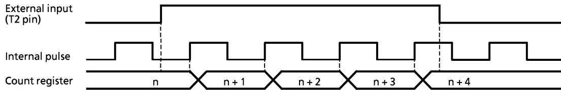
Figure 3-11. Pulse Width Measurement Mode Timing chart
