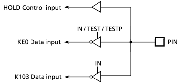
Figure 3-6. Port KE
