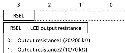
Figure 3-32. Command Register
