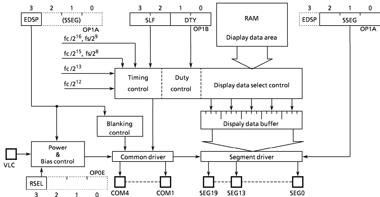
Figure 3-31. LCD Driver
