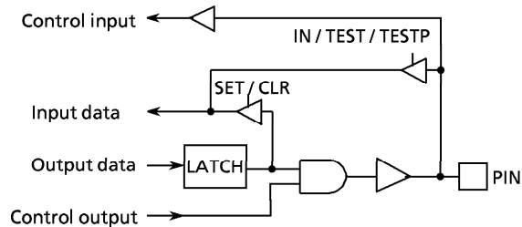
Figure 3-5. Port R9
