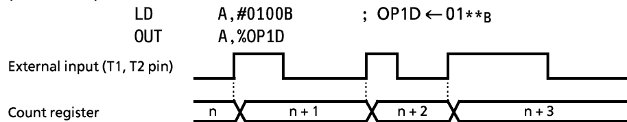
Figure 3-11. Event Counter Mode Timing Chart
