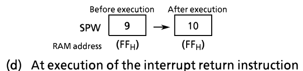
Figure 2-7. Accessing Stack (Save/Restore)
