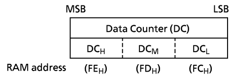
Figure 2-8. Data Counter
