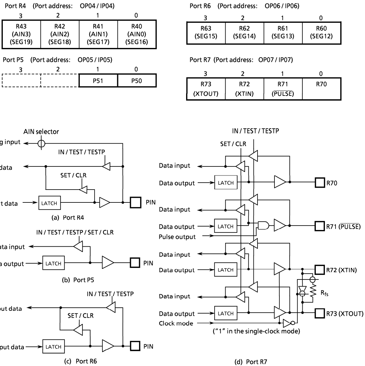
Figure 3-3. Ports R4, R5, R6 and R7
