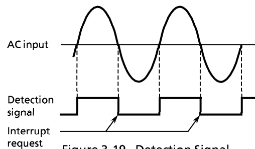
Figure 3-19. Detection Signal
