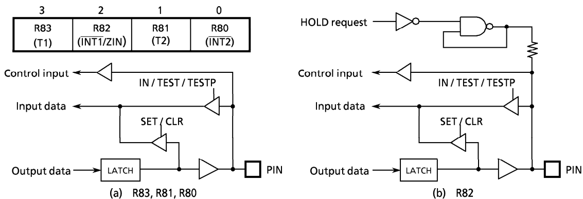
Figure 3-4. Port R8
