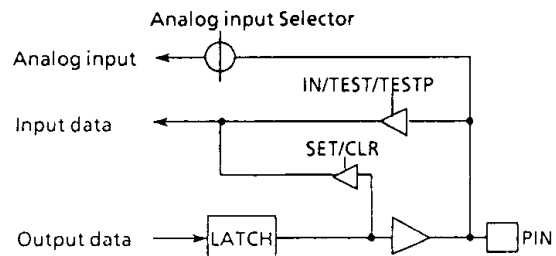
Figure 2-3. Port R4
