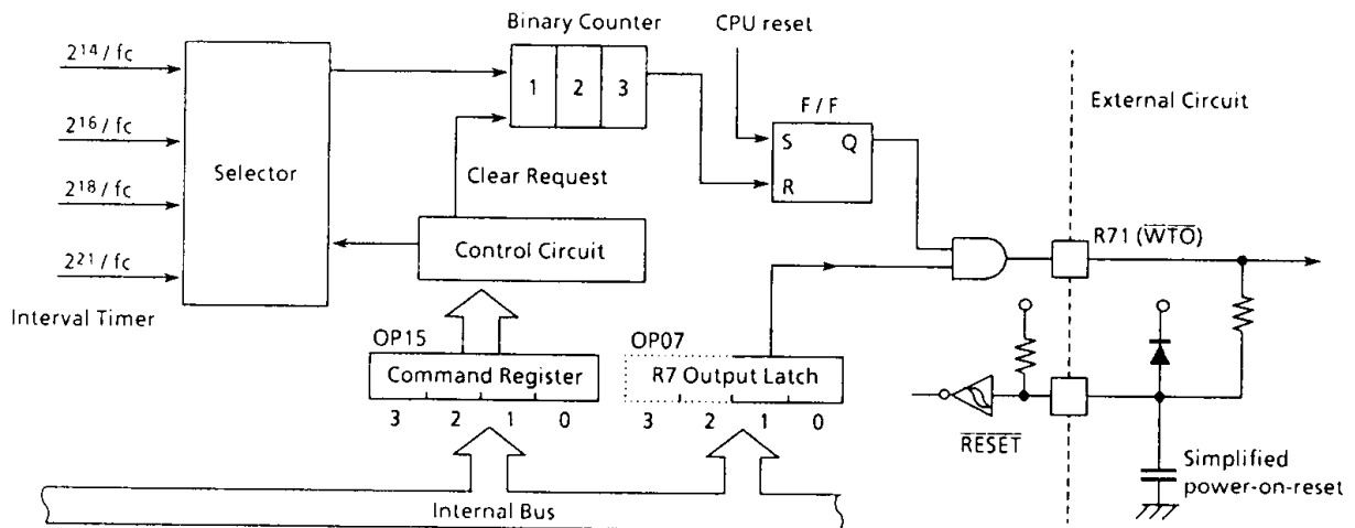
Figure 2-9. Watchdog Timer
