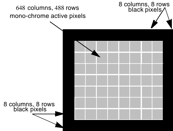
Figure 7: CMOS APS region of the LM9617
