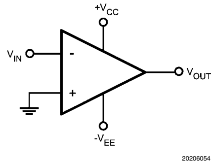
FIGURE 1. Inverting Comparator
