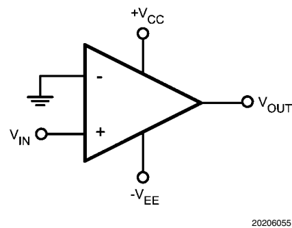
FIGURE 2. Non-Inverting Comparator
