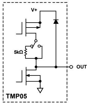
Figure 23. TMP05 One Shot Mode OUT Pin Configuration
