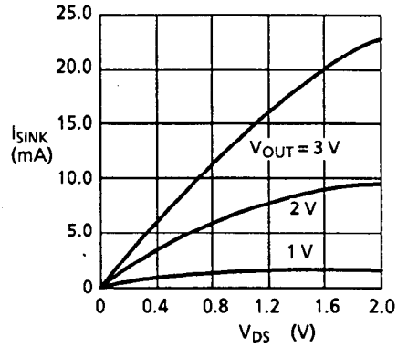
Figure 10 Sink current of Nch transistor
