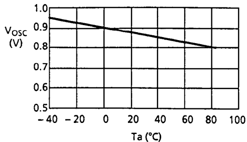
7. Oscillation start voltage - Ambient temperature
