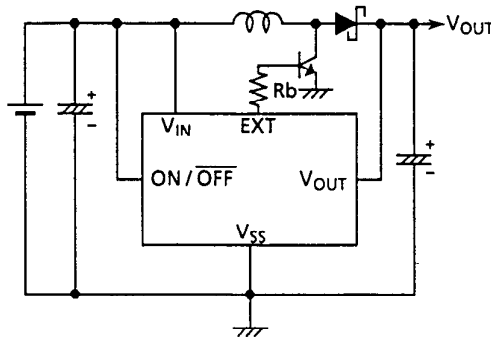
Figure 7 Circuit example with 2SC3279
