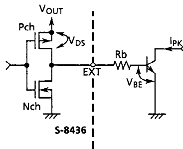
Figure 8 Peripheral circuit of external transistor
