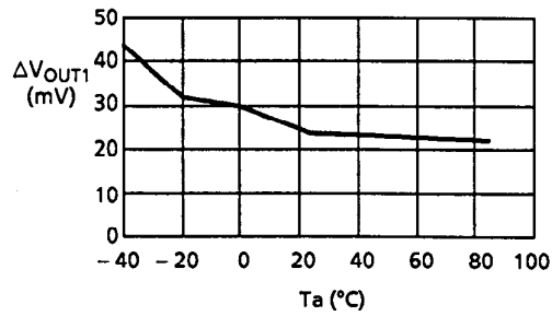
4. Output voltage - Ambient temperature
