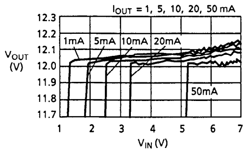
5.3 RCH855 ( L = 100 \mu\text{H} ), D1NS4, 2SC3279, R_b = 2 \text{ k}\Omega , T_a = 25^\circ\text{C}
