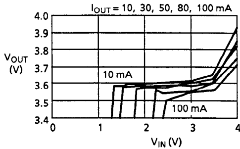
(b) V IN -V OUT
