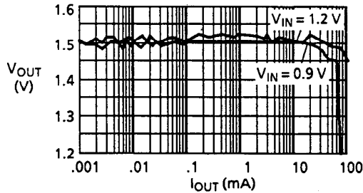
(a) I_{OUT} - V_{OUT}
