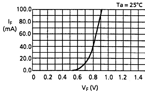
8. Forward voltage - Forward current (built-in schottky diode)
