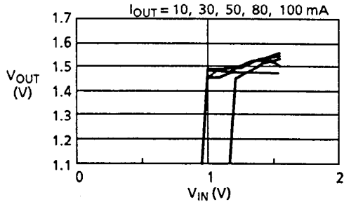
(b) V_{IN} - V_{OUT}
