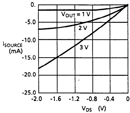
Figure 9 Source current of Pch transistor
