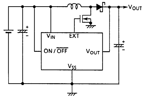
Figure 11 Example of circuit using 2SK1112
