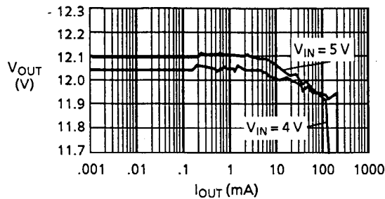
(a) I_{OUT} - V_{OUT}
