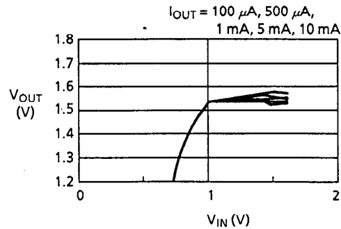
(b) V_{IN} - V_{OUT}
