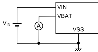
Figure 10 Test Circuit 6
