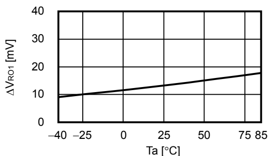
1. 11 Load Stability ( V_{RO} ) Temperature Characteristics
