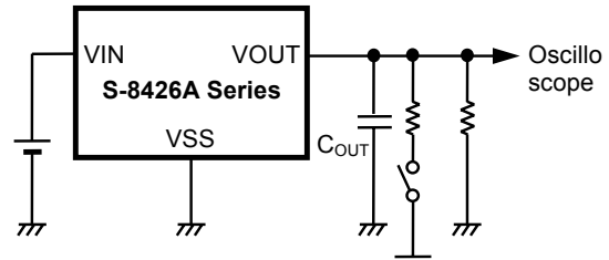
Figure 38 Test Circuit
