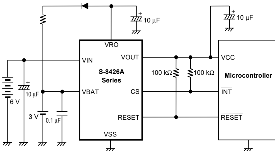
Figure 19 Application Circuit 2
