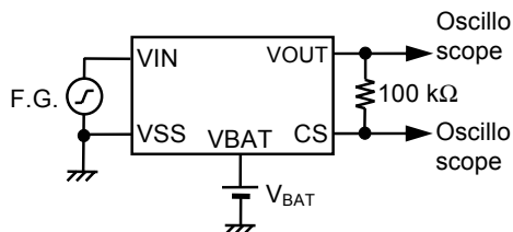
Figure 9 Test Circuit 5
