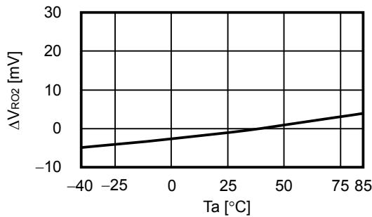
1.9 Input Stability ( V_{RO} ) Temperature Characteristics
