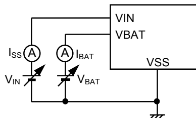
Figure 10 Test Circuit 6
