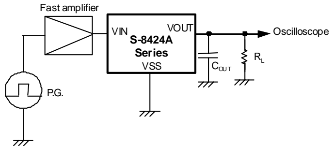
Figure 11 Test Circuit
