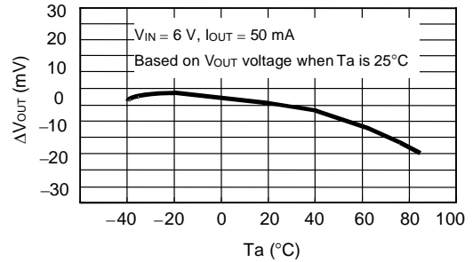
1.10 Input Stability ( V_{OUT} ) Temperature Characteristics
