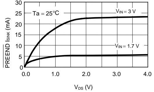
(2) Output current ( I_{SINK} ) characteristics
