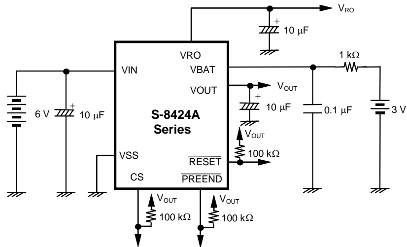
Figure 22 Standard Circuit
