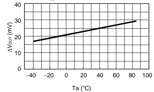
1.12 Load Stability ( V_{RO} ) Temperature Characteristics
