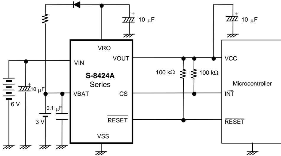
Figure 24 Application Circuit 2
