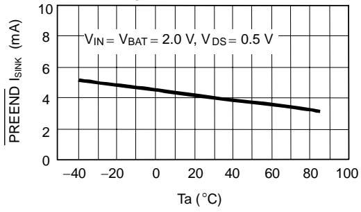
(3) Output current ( I_{SINK} ) temperature characteristics
