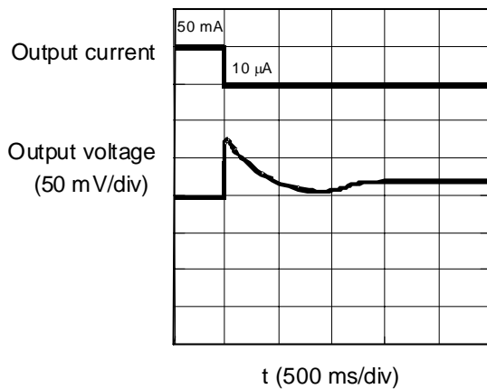
Figure 20 Ringing Waveform due to Load Variation (VOUT Pin)
