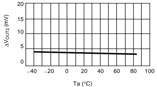
1.12 Load Stability ( V_{RO} ) Temperature Characteristics
