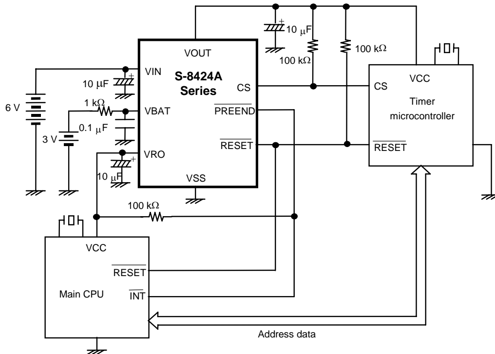
Figure 23 Application Circuit 1
