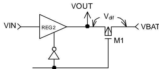
Figure 9 Definition of V_{dif}
