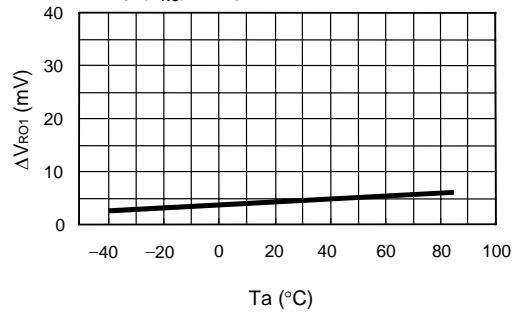
1.11 Load Stability ( V_{RO} ) Temperature Characteristics
