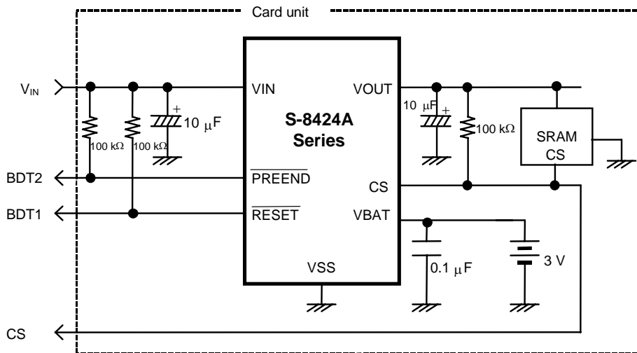
Figure 25 Application Circuit 3
