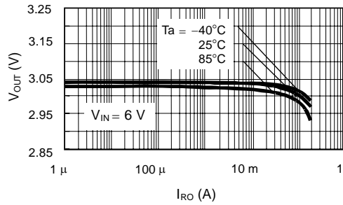
1.7 Output voltage ( V_{RO} ) Temperature Characteristics
