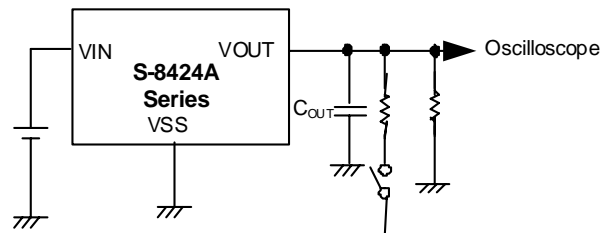
Figure 19 Test Circuit
