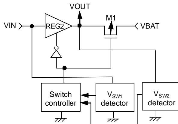
Figure 8 Switch Unit
