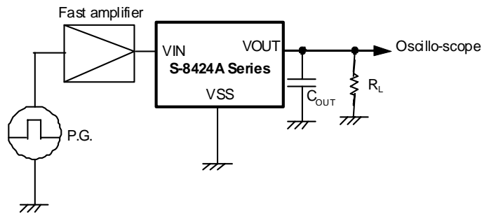
Figure 15 Test Circuit
