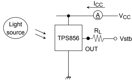
Note 5: Supply current measurement circuit
