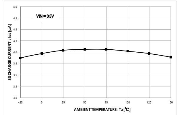
Fig.17 SS Charging current - Temperature characteristic
