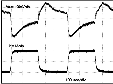
Fig.11 Output load response
