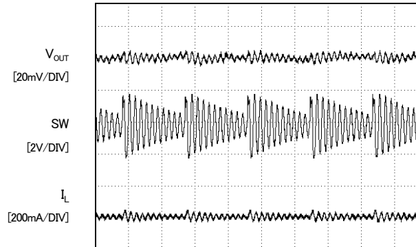
Fig.6 Low ripple mode operation
