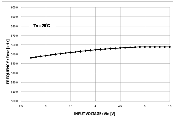
Fig.18 Switching frequency-power-supply voltage characteristic
