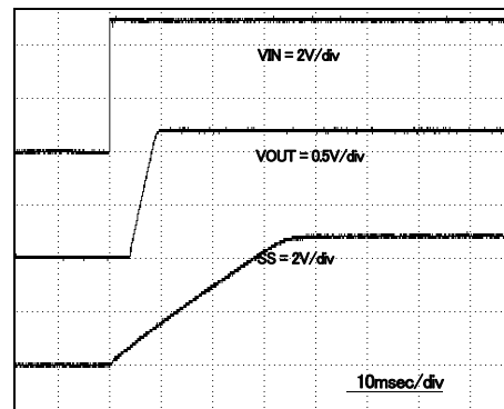
Fig.14 Soft start
