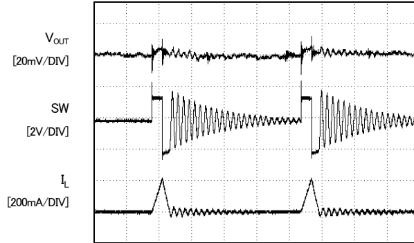
Fig.5 Low current mode operation
