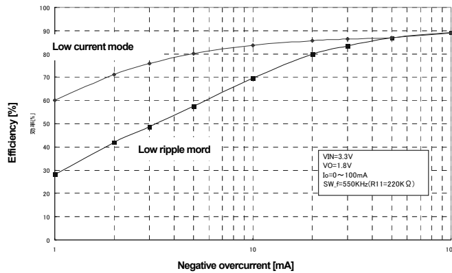
Fig7 Light load mode efficiency comparison
