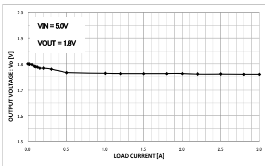
Fig.15 Regulation
