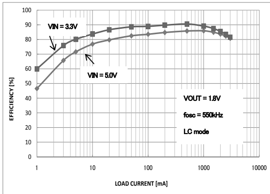
Fig.13 Efficiency
