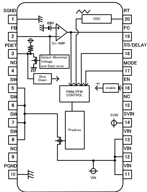
Fig1 Block diagram
