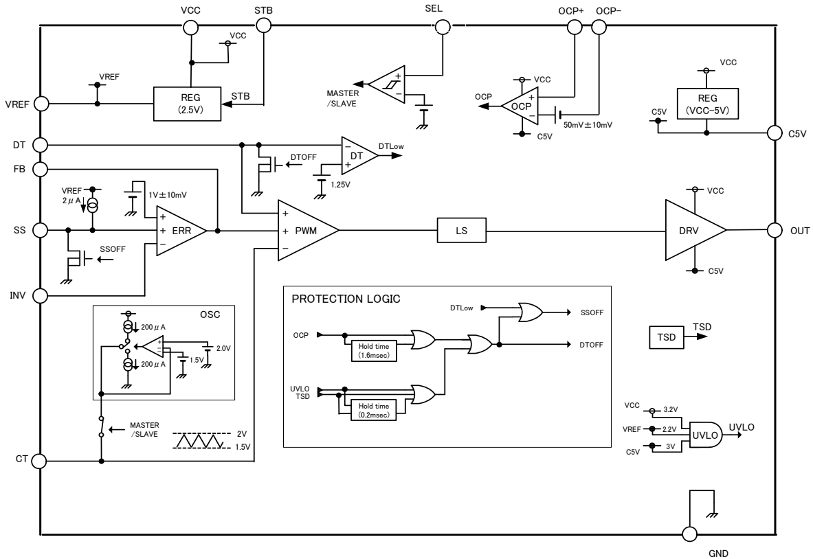
Fig.28 Block diagram
