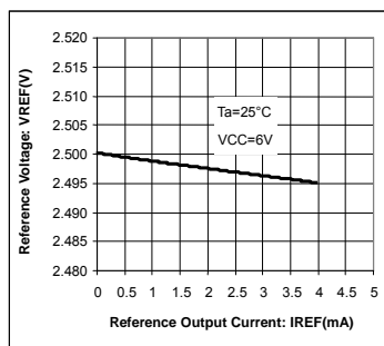
Fig.5 VREF current capability
