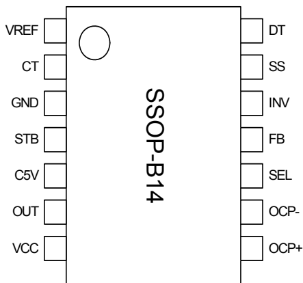
Fig.29 Pin layout
