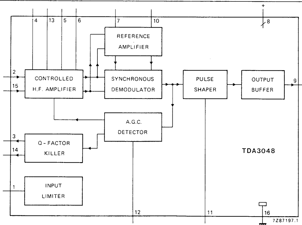
Fig. 1 Block diagram of TDA3048.
