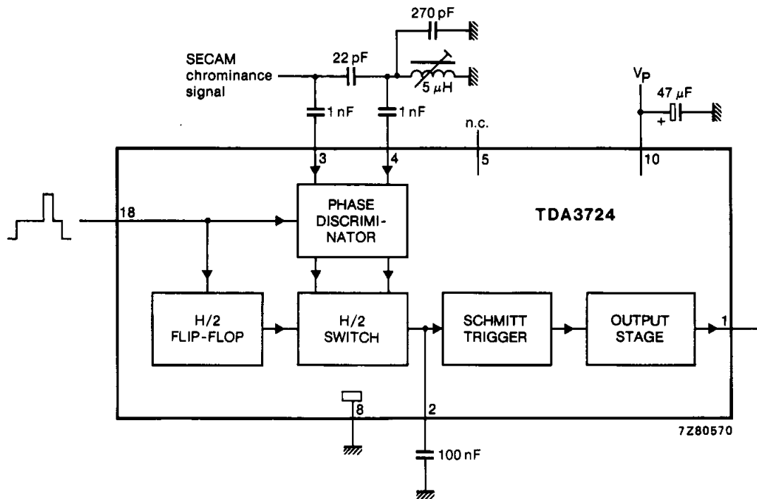
Fig. 1 Block diagram.
