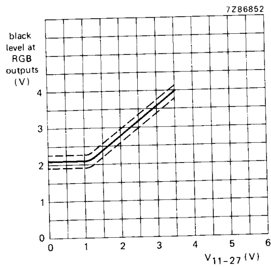
Fig. 4 Brightness control voltage range.
