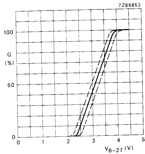
Fig. 3 Saturation control voltage range.
