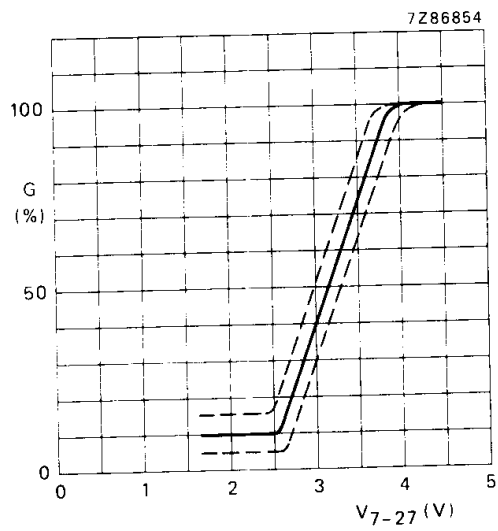
Fig. 2 Contrast control voltage range.
