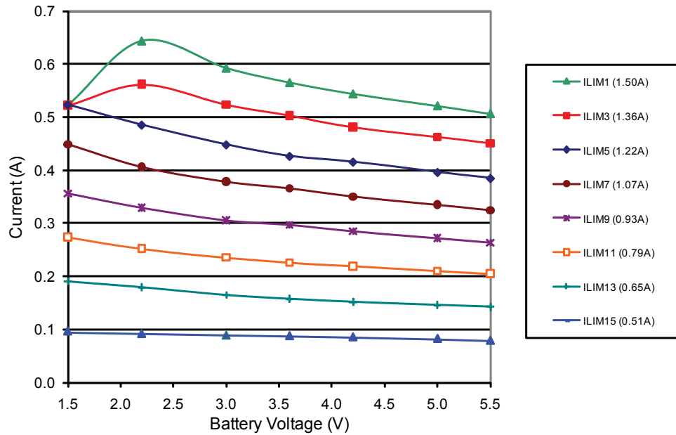
Average Input Current versus Battery Voltage at Various ILIM
