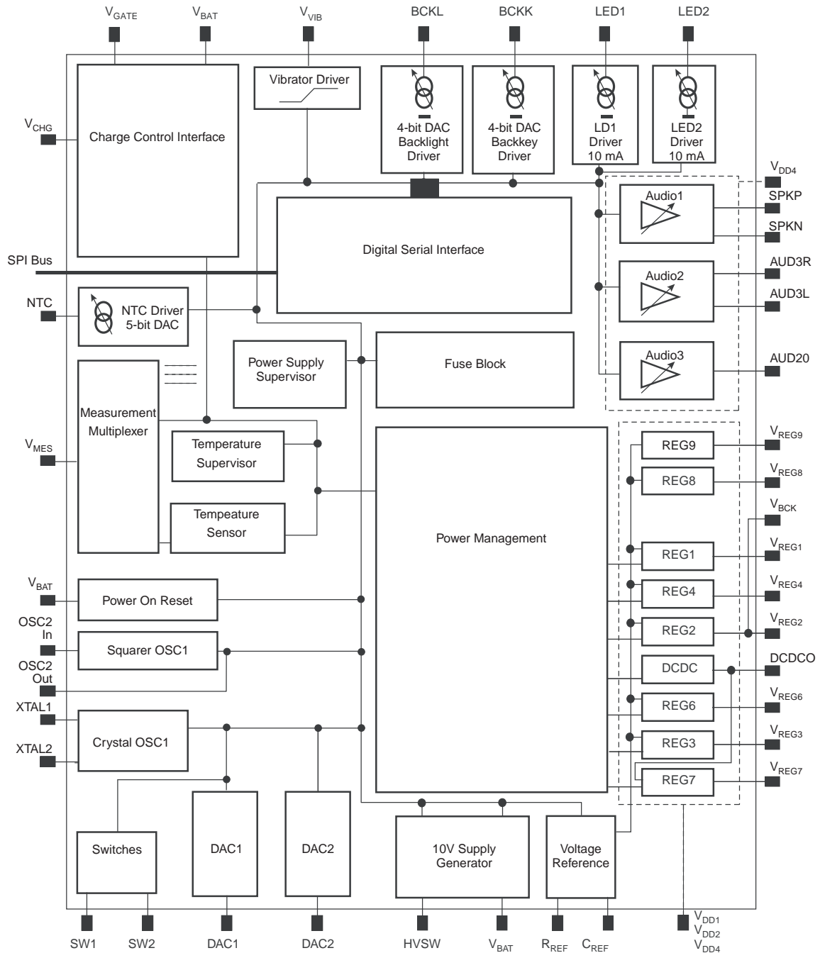
Figure 1. AT73C201 Functional Diagram
