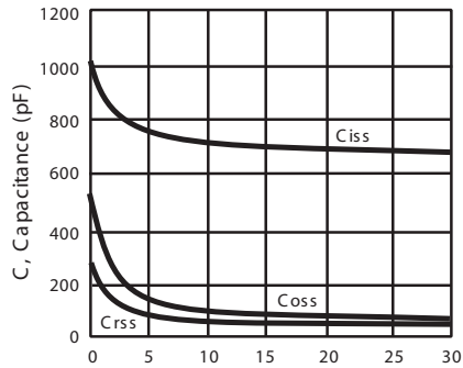
Figure 9. Capacitance
