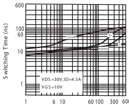
Figure 11. switching characteristics
