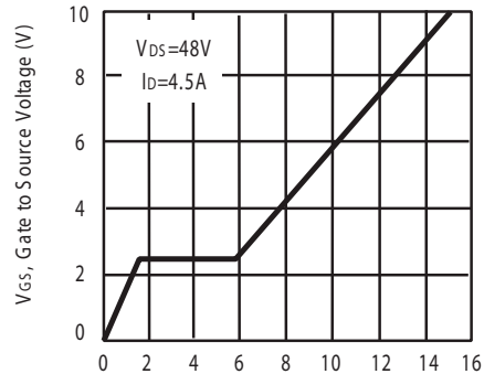
Figure 10. Gate Charge
