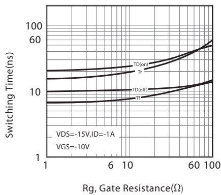
Figure 11. switching characteristics
