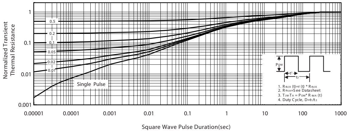
Figure 14. Normalized Thermal Transient Impedance Curve
