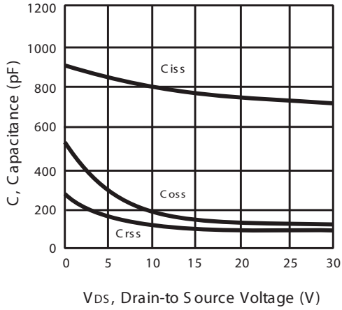
Figure 9. Capacitance
