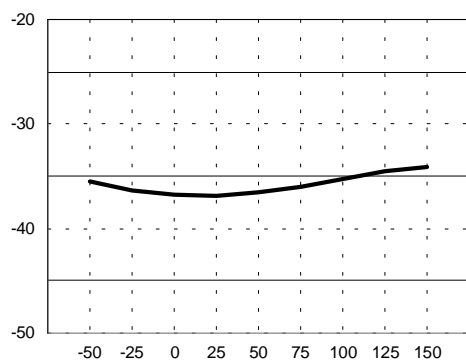
Figure 9. -12V bias current
