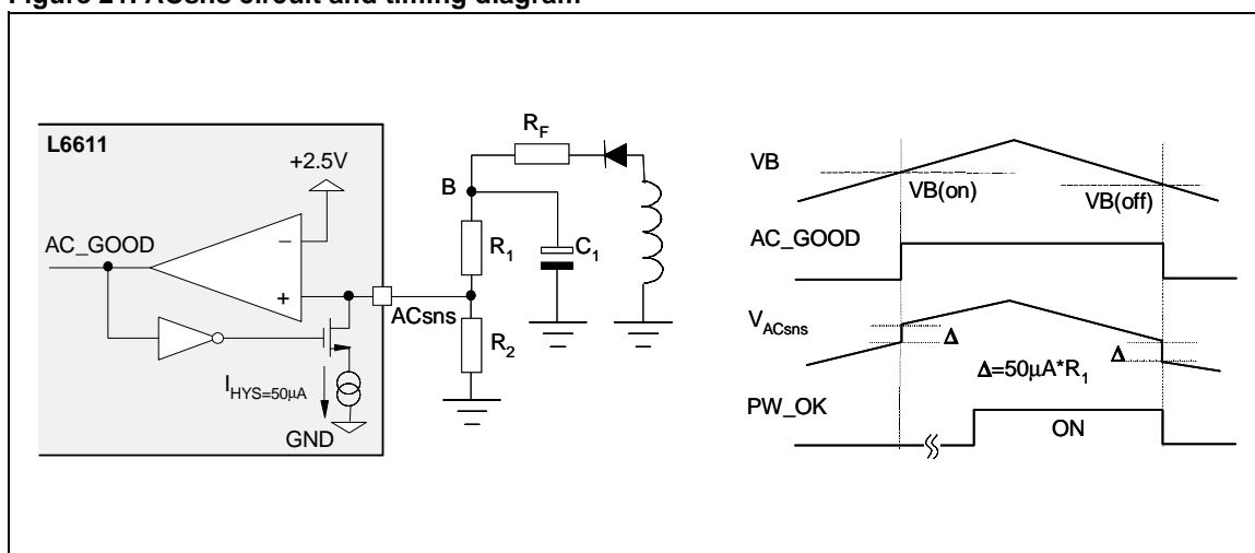
Figure 21. ACsns circuit and timing diagram
