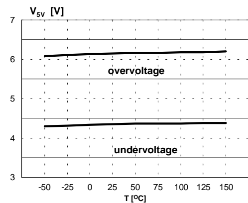
Figure 6. 5V fault thresholds
