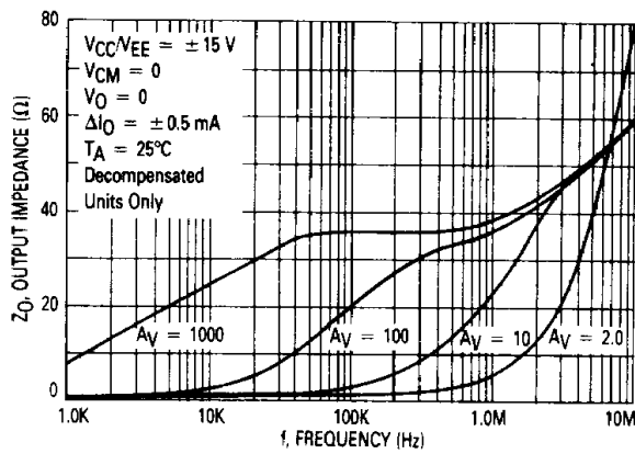
FIGURE 10 — OUTPUT IMPEDANCE versus FREQUENCY
