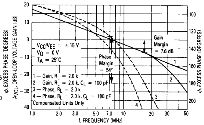
FIGURE 15 — OPEN-LOOP VOLTAGE GAIN AND PHASE versus FREQUENCY
