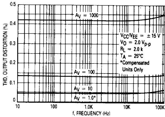
FIGURE 12 — OUTPUT DISTORTION versus FREQUENCY
