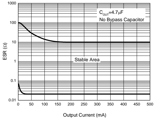
Figure 20. ESR vs. Output Current
