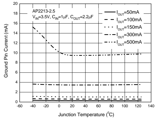
Figure 7. Ground Pin Current vs. Junction Temperature
