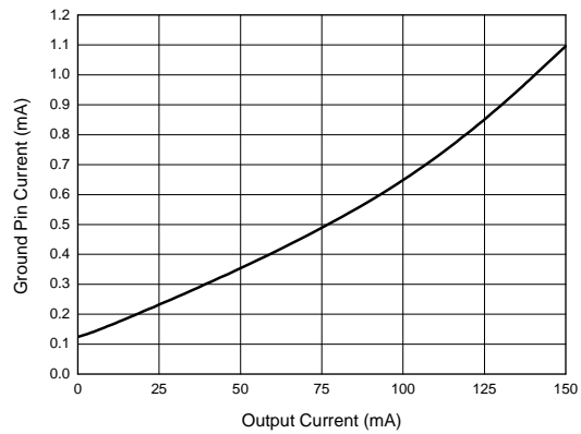
Figure 6. Ground Pin Current vs. Output Current
