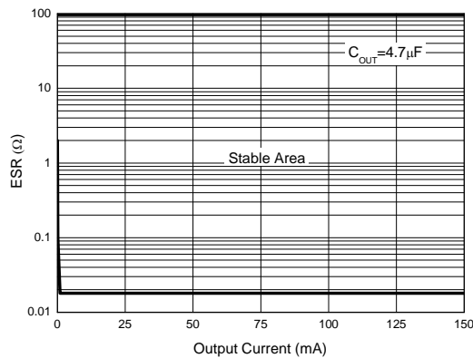
Figure 18. ESR vs. Output Current
