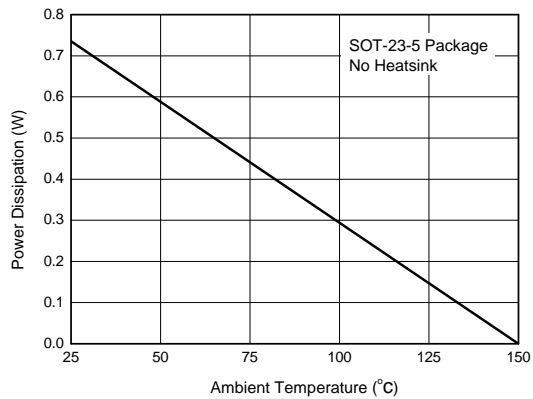
Figure 15. Power Dissipation vs. Ambient Temperature
