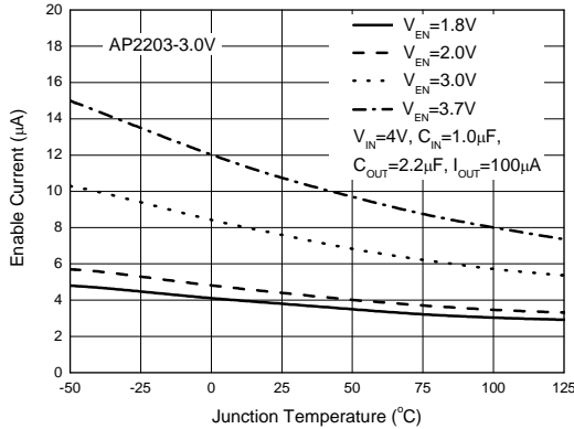
Figure 8. Enable Current vs. Junction Temperature
