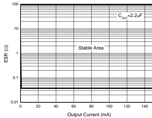
Figure 17. ESR vs. Output Current
