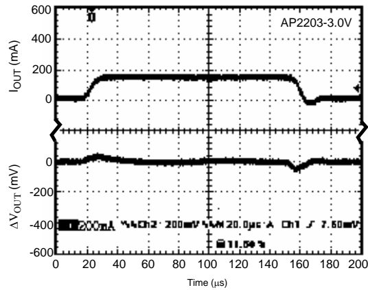
Figure 11. Load Transient (Conditions: V IN =4V, V EN =2V, I OUT =5mA to 200mA, C IN =1µF, C OUT =2.2µF)
