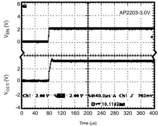
Figure 13. V_{EN} (on) vs. V_{OUT} (Conditions: V_{EN} =0 to 2V, V_{IN} =4V, I_{OUT} =30mA, C_{IN} =1.0 \mu F, C_{OUT} =2.2 \mu F)
