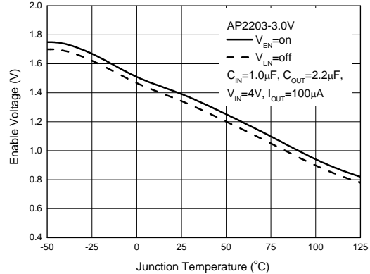
Figure 9. Enable Voltage vs. Junction Temperature
