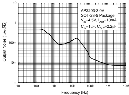
Figure 10. Output Noise vs. Frequency
