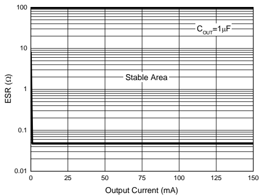
Figure 16. ESR vs. Output Current
