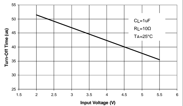
Turn-Off Time vs Input Voltage
