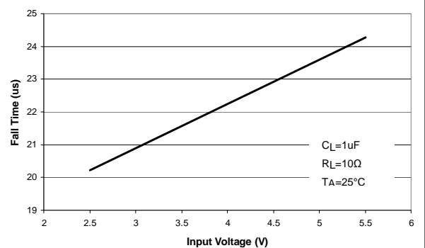
Fall Time vs Input Voltage
