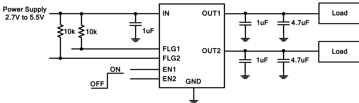
AP2152A Enable Active High
