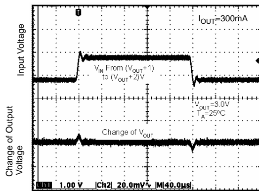
Figure 16. Line Transient
