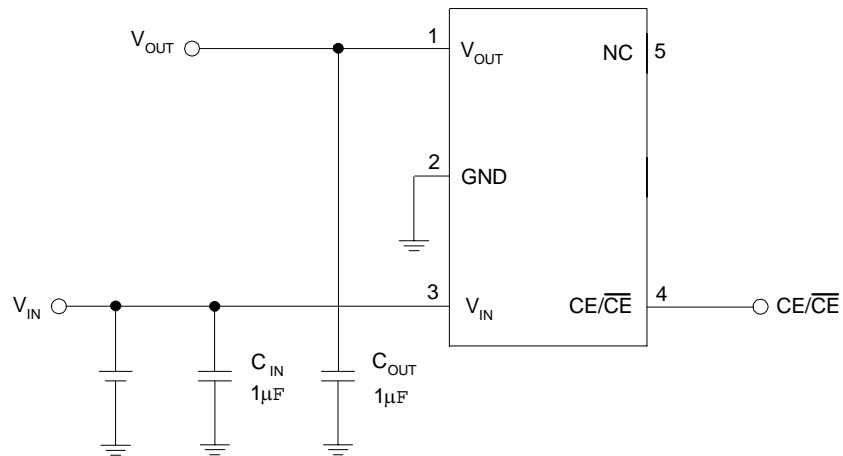
Figure 17. Typical Application of AP2115
