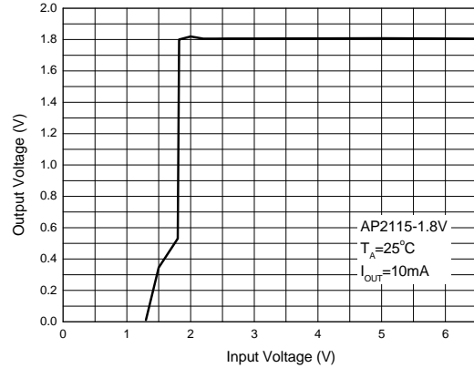
Figure 5. Output Voltage vs. Input Voltage
