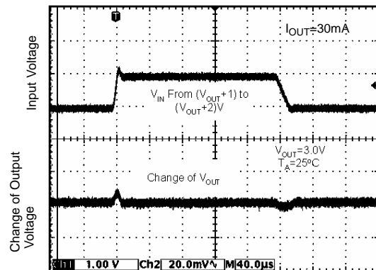
Figure 15. Line Transient
