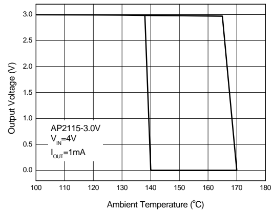
Figure 13. Output Voltage vs. Ambient Temperature
