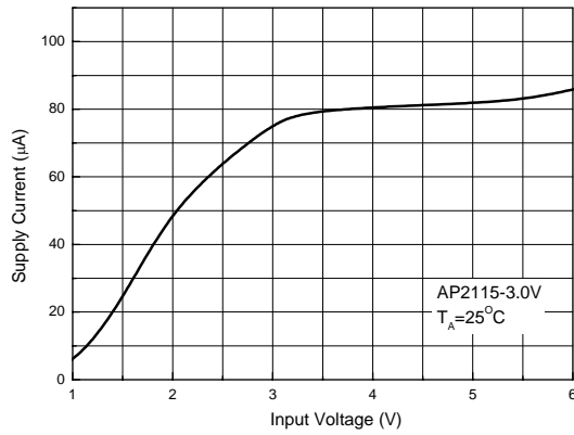
Figure 8. Input Voltage vs. Supply Current (No Load)
