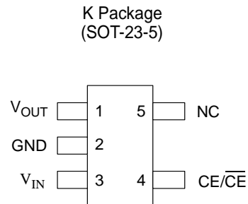
Figure 2. Pin Configuration of AP2115 (Top View)
