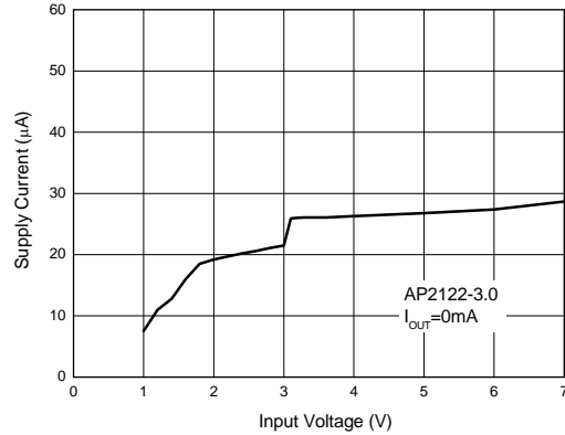
Figure 13. Supply Current vs. Input Voltage
