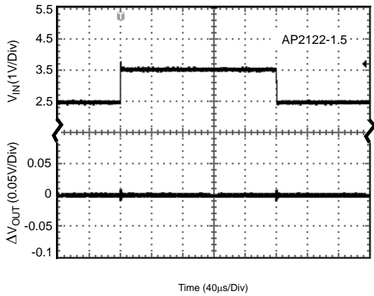
Figure 16. Line Transient (Conditions: I_{OUT}=30\text{mA} , C_{IN}=1\mu\text{F} , C_{OUT}=1\mu\text{F} )
