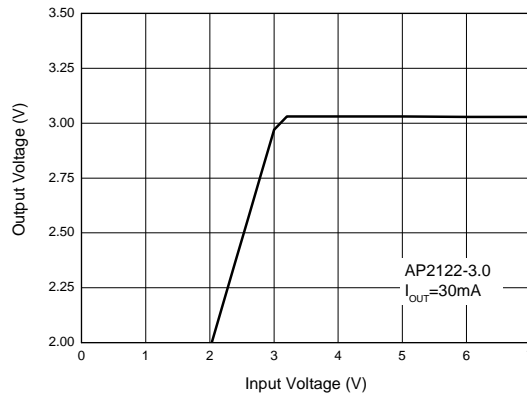
Figure 7. Output Voltage vs. Input Voltage
