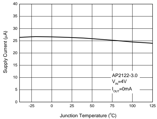
Figure 15. Supply Current vs. Junction Temperature
