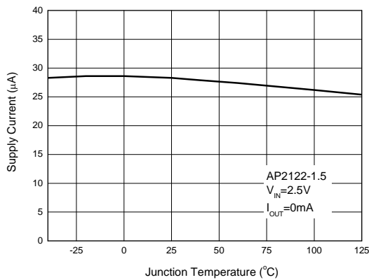
Figure 14. Supply Current vs. Junction Temperature
