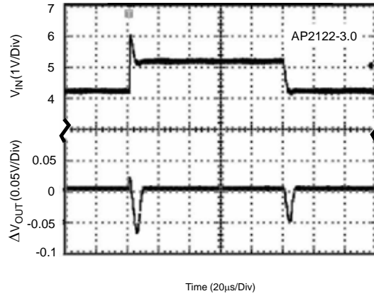
Figure 17. Line Transient (Conditions: I_{OUT}=30\text{mA} , C_{IN}=1\mu\text{F} , C_{OUT}=1\mu\text{F} )
