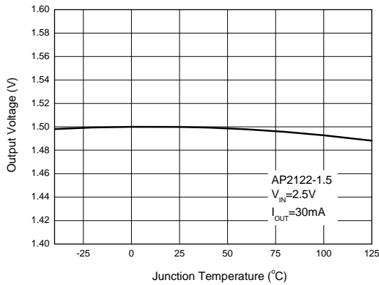
Figure 10. Output Voltage vs. Junction Temperature
