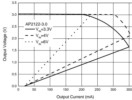
Figure 5. Output Voltage vs. Output Current
