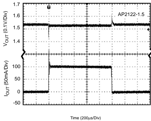
Figure 18. Load Transient (Conditions: V_{IN}=2.5\text{V} , C_{IN}=1\mu\text{F} , C_{OUT}=1\mu\text{F} )
