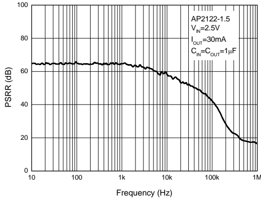
Figure 20. PSRR vs. Frequency
