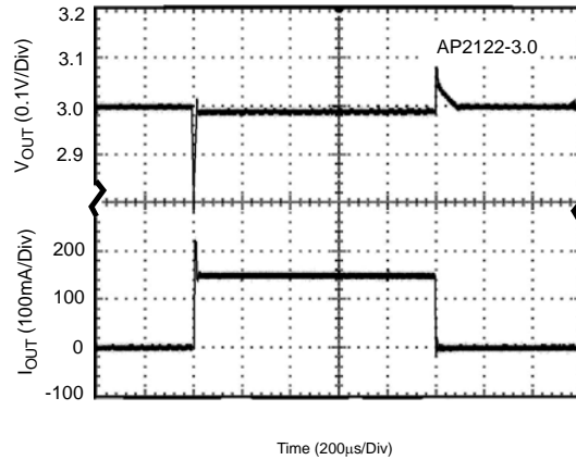
Figure 19. Load Transient (Conditions: V_{IN}=4\text{V} , C_{IN}=1\mu\text{F} , C_{OUT}=1\mu\text{F} )
