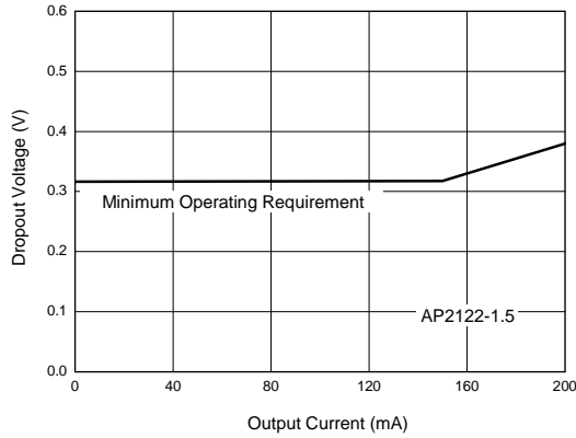
Figure 8. Dropout Voltage vs. Output Current
