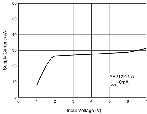
Figure 12. Supply Current vs. Input Voltage
