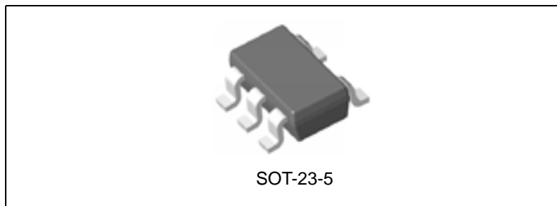
Figure 1. Package Type of AP2122
