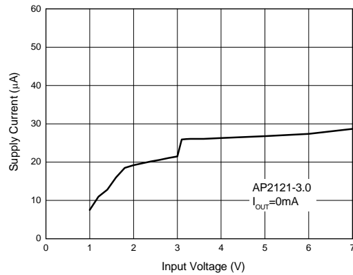
Figure 13. Supply Current vs. Input Voltage
