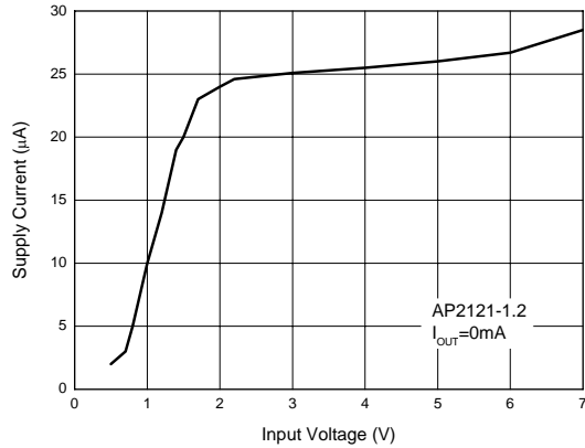
Figure 12. Supply Current vs. Input Voltage
