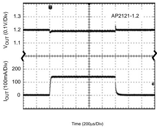
Figure 18. Load Transient (Conditions: V_{IN}=2.2\text{V} , C_{IN}=1\mu\text{F} , C_{OUT}=1\mu\text{F} )
