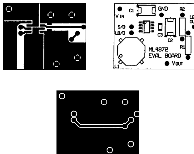
Figure 8. Sample PC Board Layout
