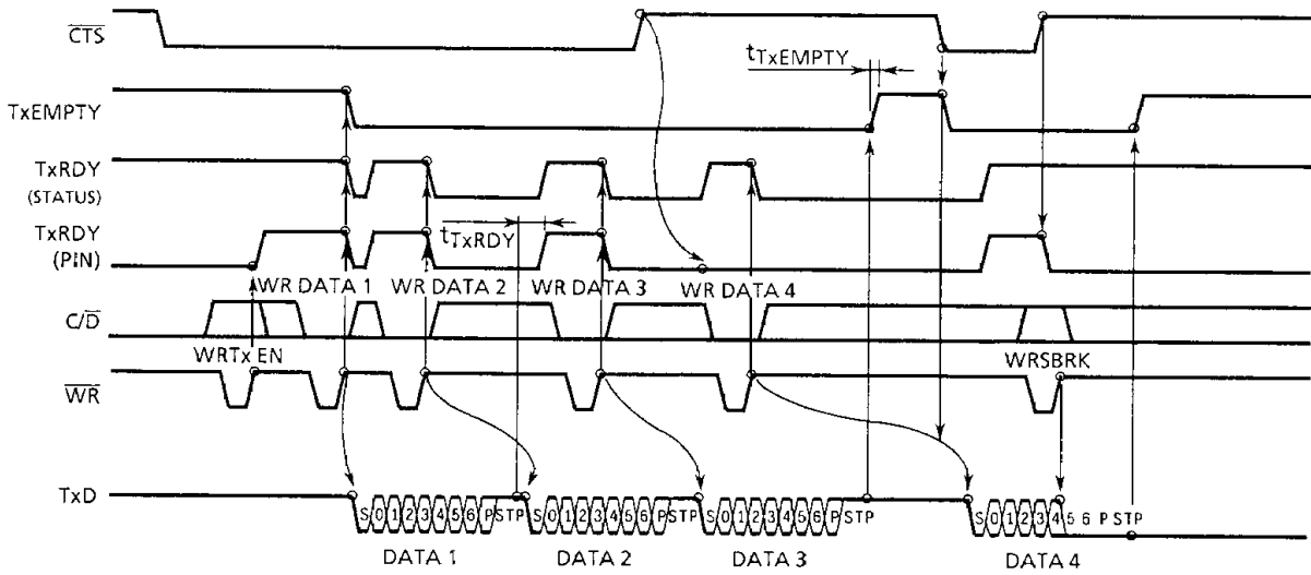
EXAMPLE FORMAT : 7 BIT CHARACTER & 2 STOP BITS.
