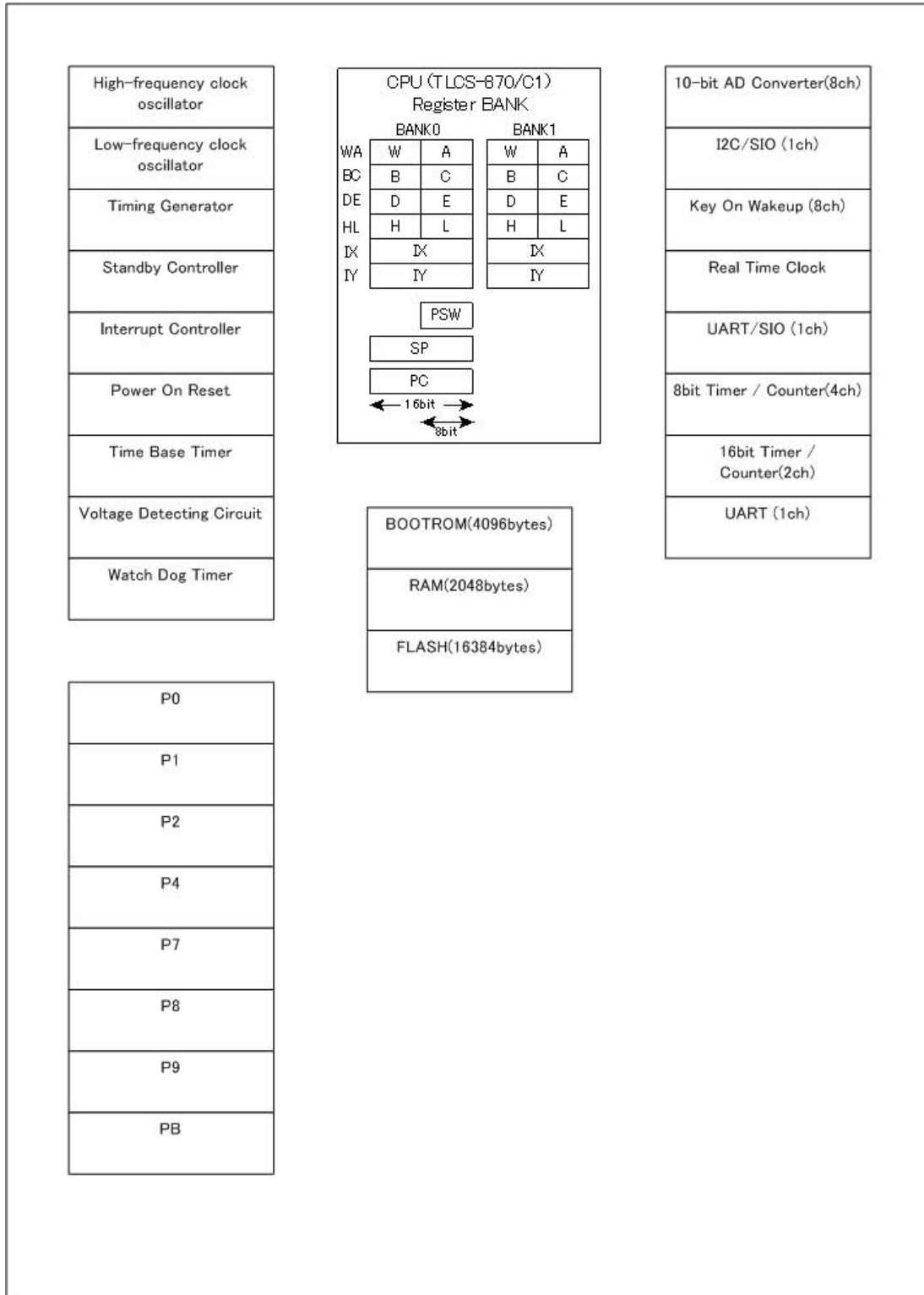
Figure 1-2 Block Diagram
