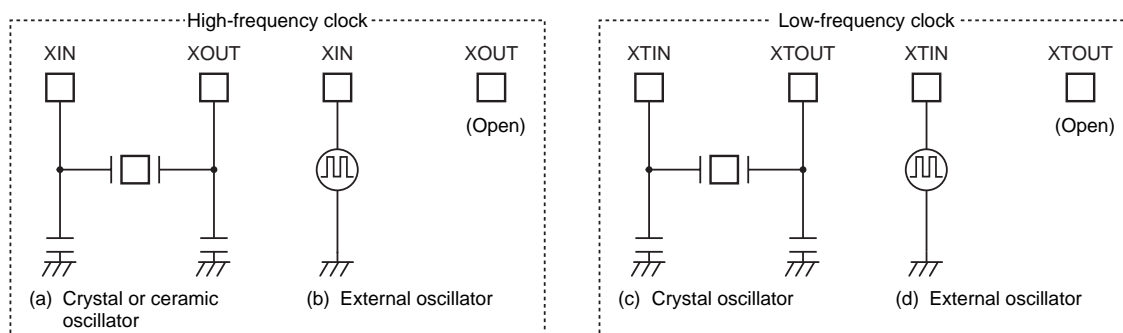
Figure 2-4 Examples of Oscillator Connection
