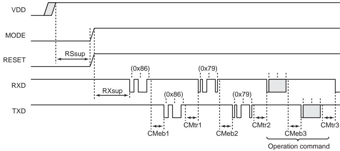
Figure 22-6 Reset Timing
