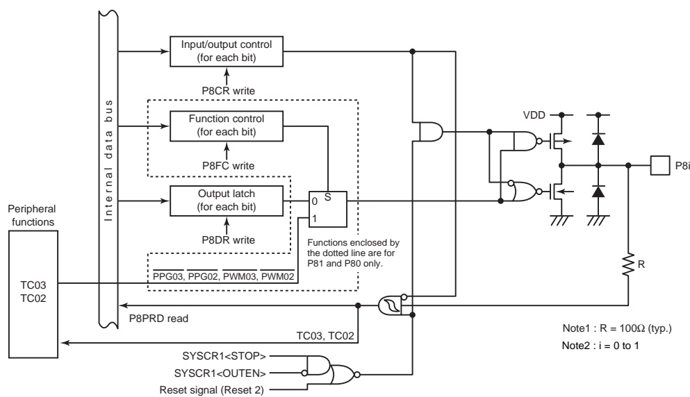
Figure 8-8 Port P8
