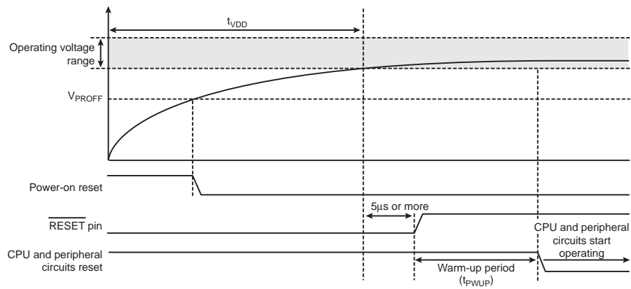
Figure 2-15 External Reset Input (During Power-Up)
