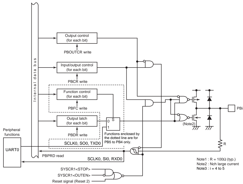
Figure 8-10 Port PB
