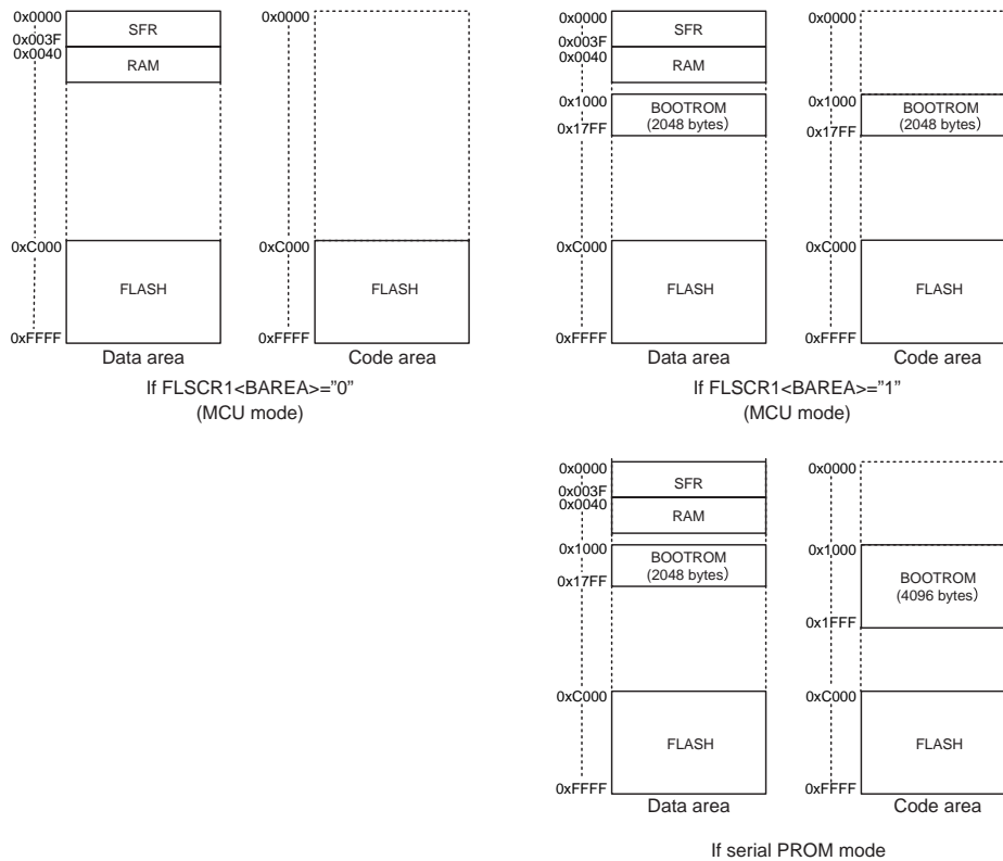
Figure 22-3 Memory Mapping
