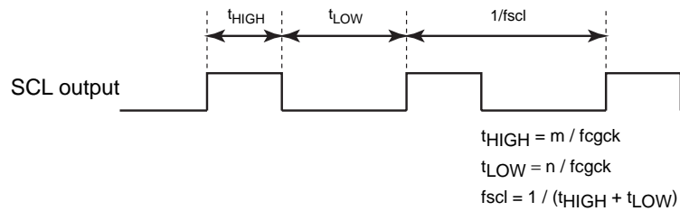
Figure 18-6 SCL Output
