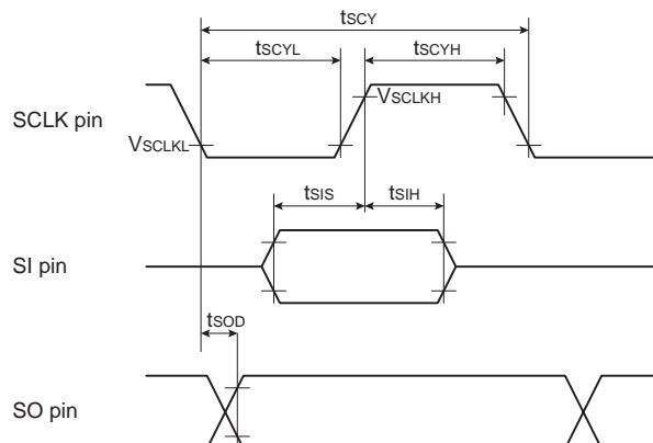
Figure 17-17 AC Characteristics
