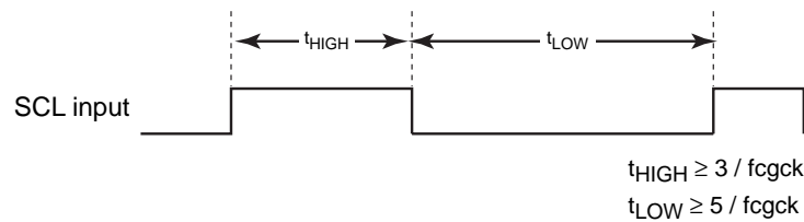
Figure 18-7 SCL Input
