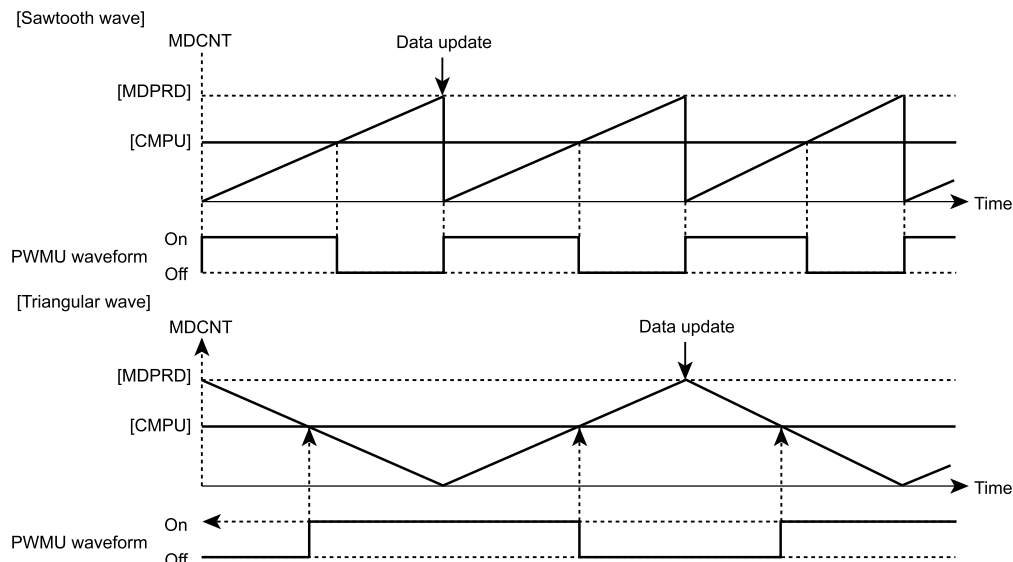
Figure 14-9 PWM Waveforms
