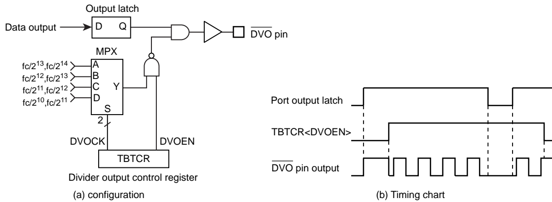
Figure 8-3 Divider Output
