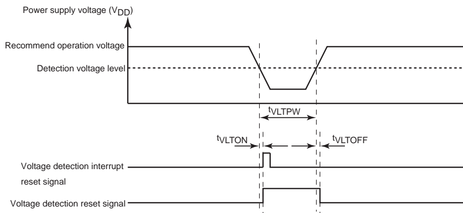
Figure 21-3 Operation timing of Voltage detection circuit
