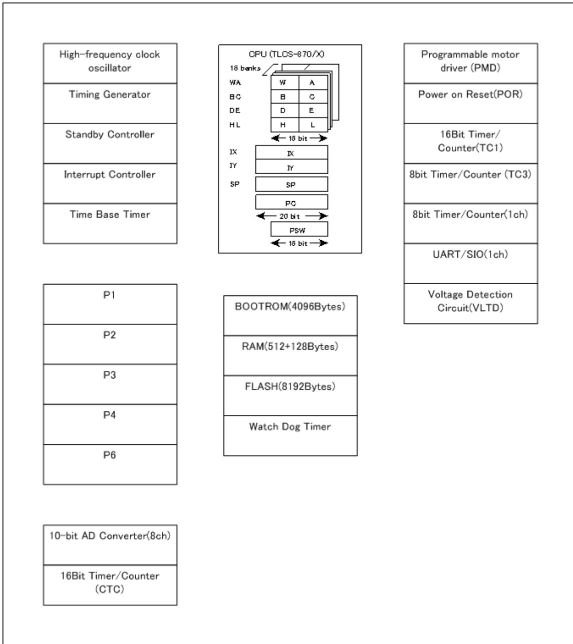
Figure 1-2 Block Diagram
