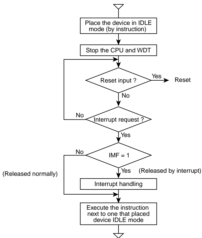
Figure 2-9 IDLE Mode
