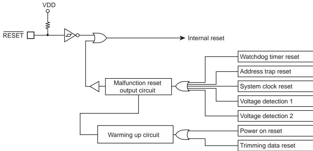
Figure 2-11 Reset Circuit
