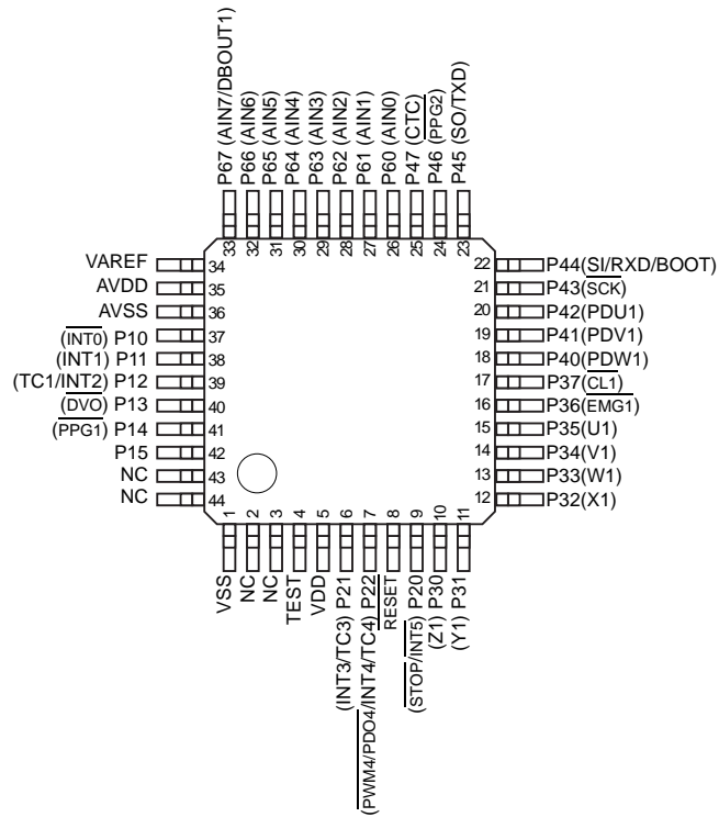
Figure 1-1 Pin Assignment
