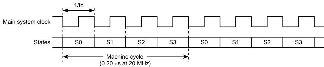
Figure 2-4 Machine Cycles
