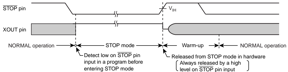
Figure 2-6 Released from STOP Mode by Level
