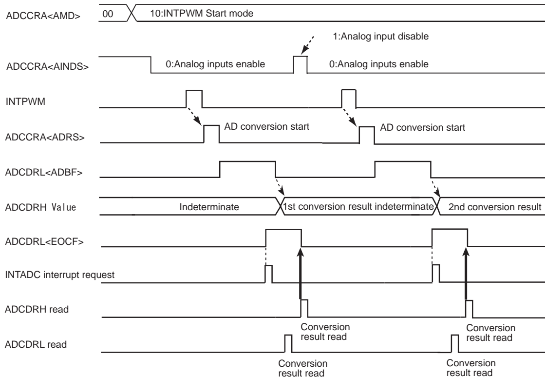
Figure 17-4 INTPWM Start Mode
