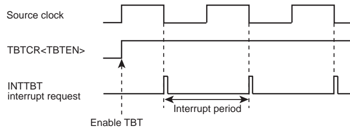
Figure 8-2 Time Base Timer Interrupt
