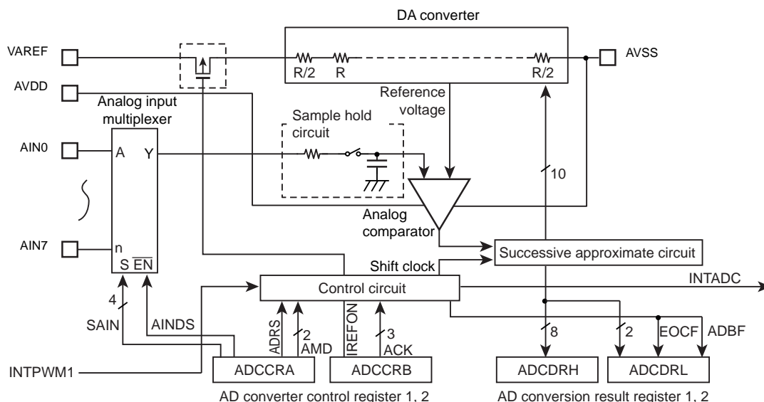
Figure 17-1 10-bit AD Converter
