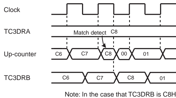
Figure 12-2 Auto-Capture Function
