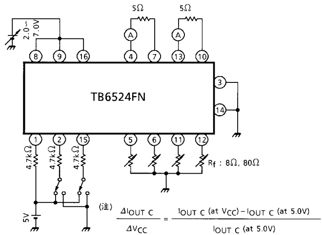
TEST CIRCUIT 5 \Delta I_{OUT\ C}
