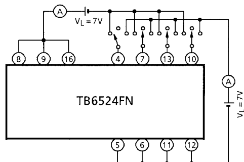
TEST CIRCUIT 8 I_{LU} / I_{LL}
