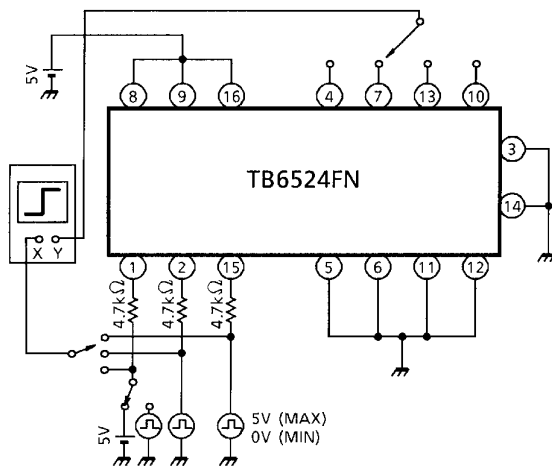
TEST CIRCUIT 8 I_{LU} / I_{LL}
