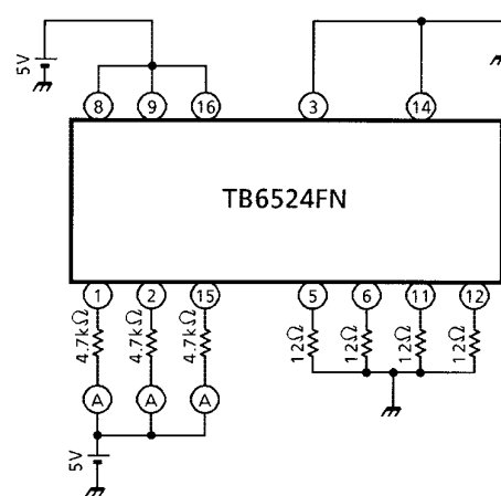
TEST CIRCUIT 7 I_{in}
