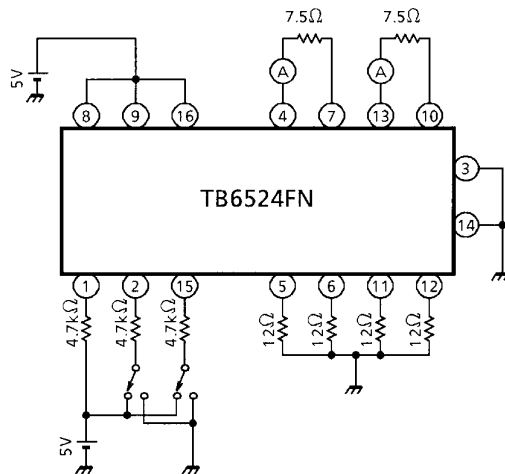
TEST CIRCUIT 4 I_{OUT\ C}
