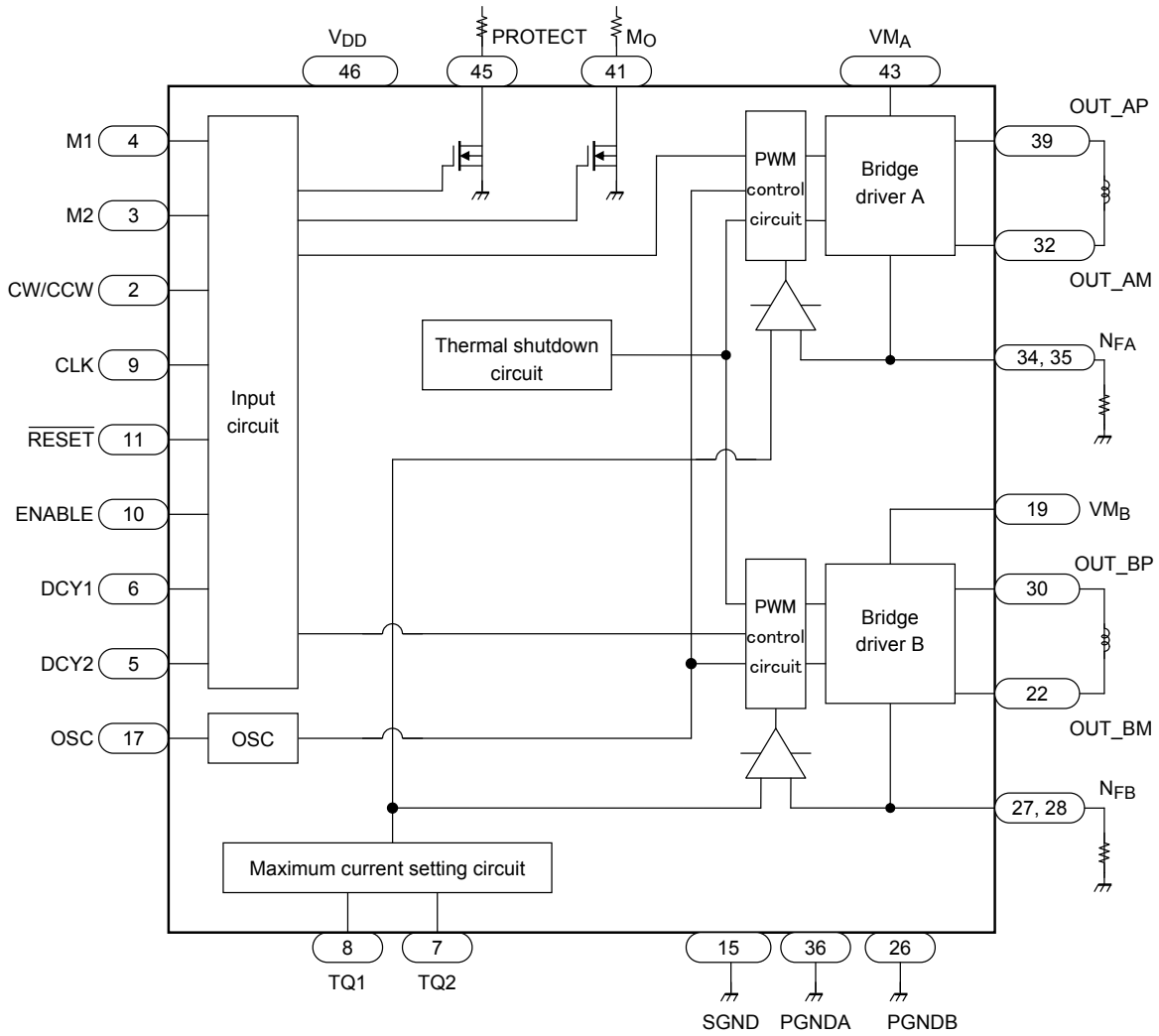
TB6560AFTG
