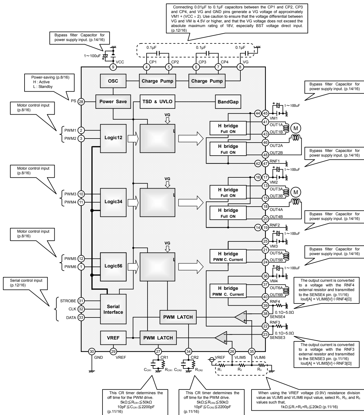
Fig.20 BD6753KV Application Circuit Diagram
