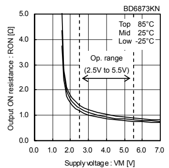
Fig.9 Output ON-Resistance (Linear Constant-Current Drive)
