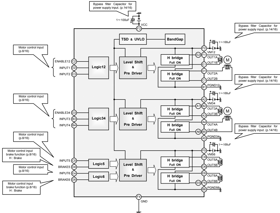
Fig.18 BD6373GW Application Circuit Diagram
