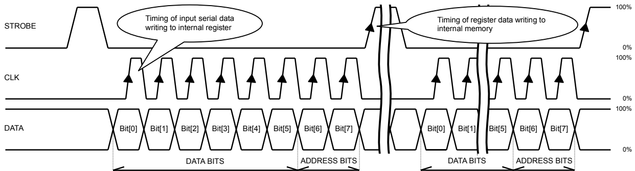
Fig.22 BD6753KV Sequence of Serial Control Input
