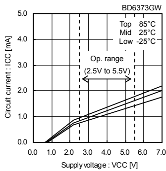
Fig.4 Circuit current
