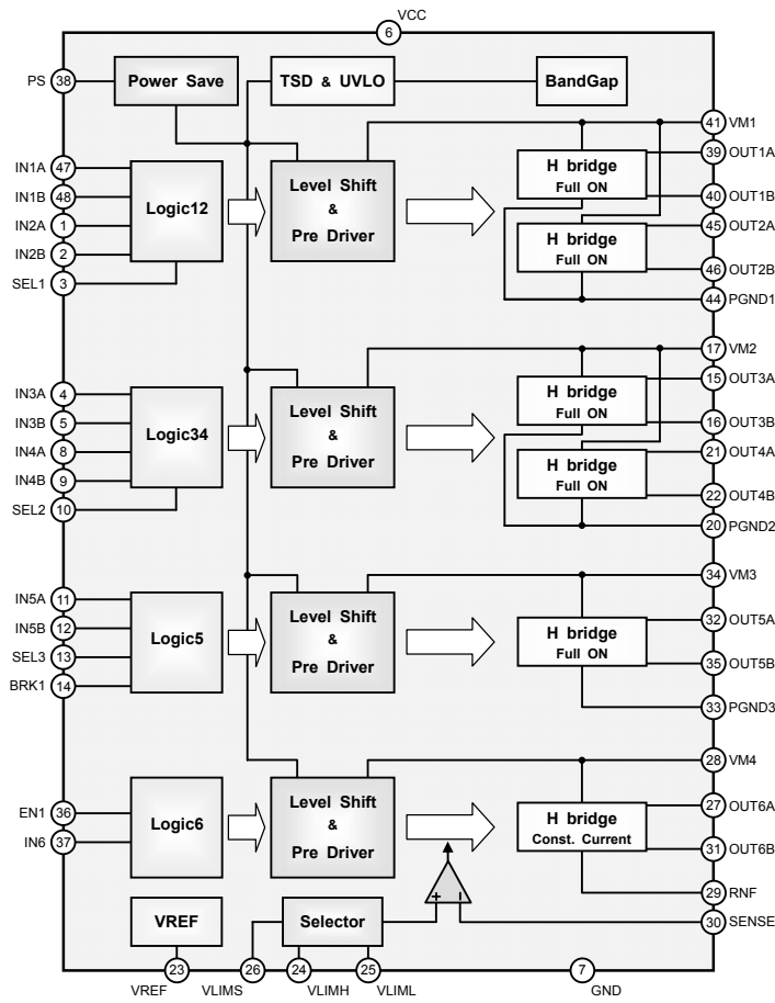
Fig. 14 BD6873KN Block Diagram
