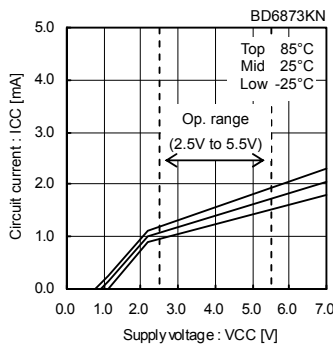
Fig.5 Circuit current
