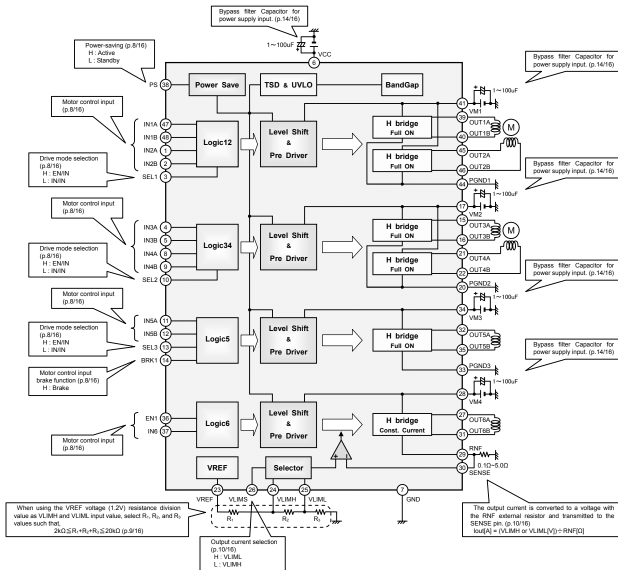
Fig.19 BD6873KN Application Circuit Diagram
