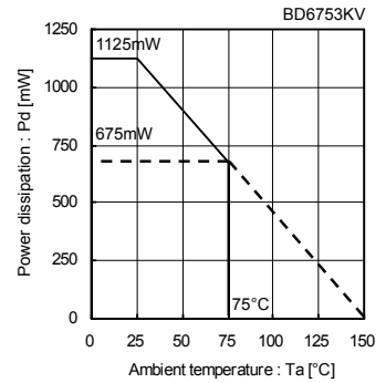
Fig.3 Power Dissipation Reduction
