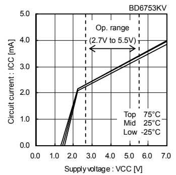
Fig.6 Circuit current
