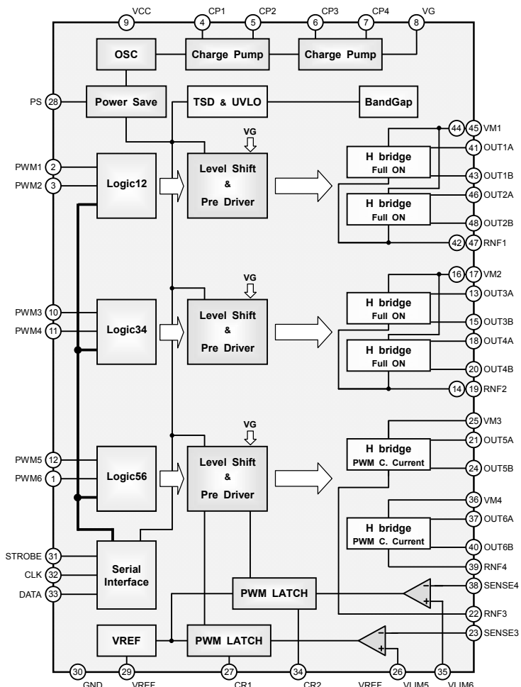
Fig.16 BD6753KV Block Diagram
