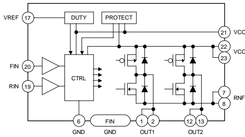
Fig.29 BD6222FP
