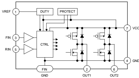
Fig.27 BD6220/21/22HFP
