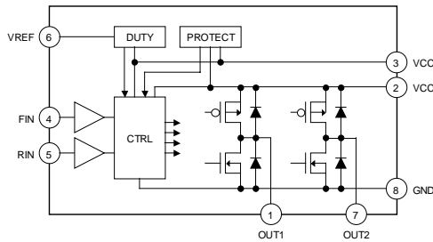
Fig.25 BD6220F / BD6221F
