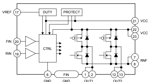
Fig.29 BD6222FP
