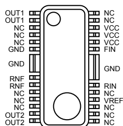
Fig.30 HSOP25
