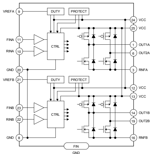
Fig.31 BD6225FP / BD6226FP
