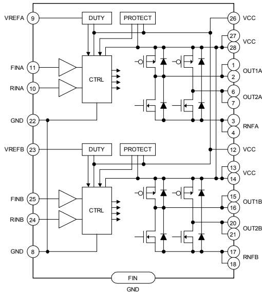
Fig.35 BD6227FM
