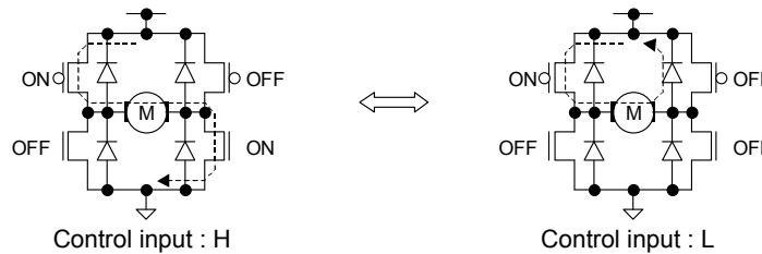
Fig.38 PWM control operation (output stage)
