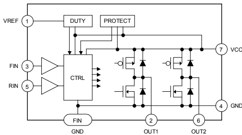
Fig.27 BD6230HFP / BD6231HFP / BD6232HFP
