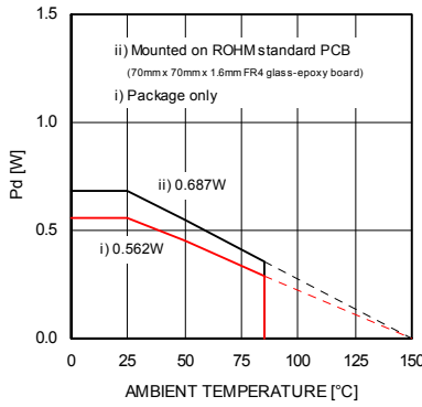
Fig.42 Thermal derating curve (SOP8)
