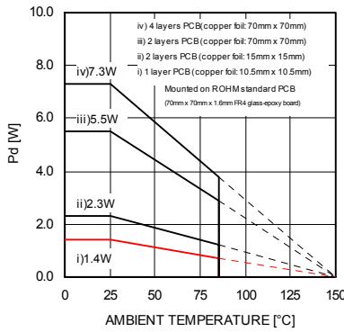
Fig.45 Thermal derating curve (HRP7)
