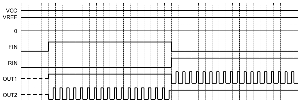
Fig.40 VREF control operation (timing chart)
