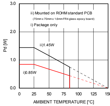
Fig.43 Thermal derating curve (HSOP25)
