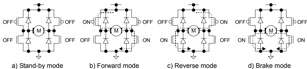
Fig.37 Four basic operations (output stage)
