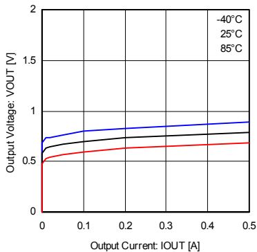
Fig.22 Low side body diode (0.5A class)
