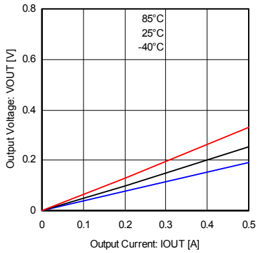
Fig.19 Output low voltage (0.5A class)
