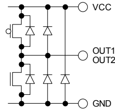
Fig.48 OUT1 / OUT2 (SOP8/HRP7)
