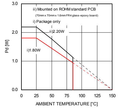
Fig.44 Thermal derating curve (HSOP-M28)
