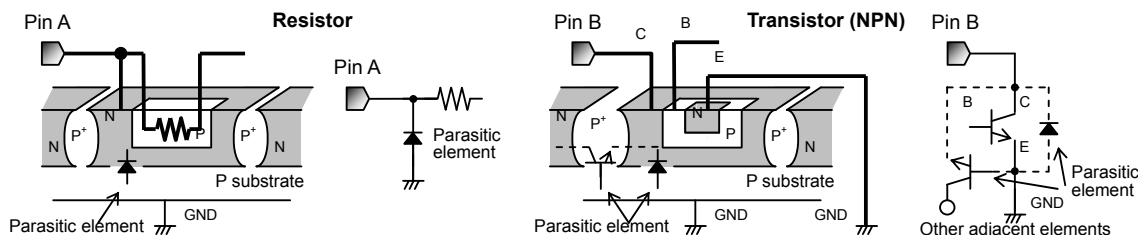
Appendix: Example of monolithic IC structure
