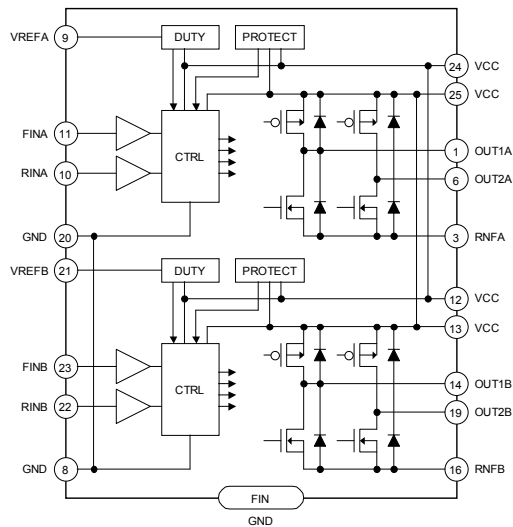
Fig.31 BD6235FP / BD6236FP
