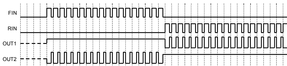
Fig.39 PWM control operation (timing chart)
