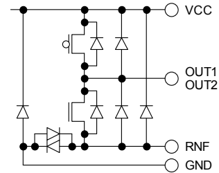
Fig.49 OUT1 / OUT2 (HSOP25/HSOPM28)
