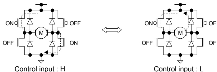
Fig.38 PWM control operation (output stage)
