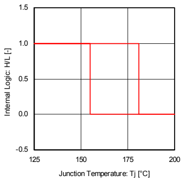
Fig.10 Thermal shutdown
