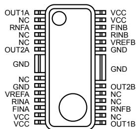
Fig.32 HSOP25
