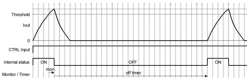
Fig.41 Over current protection (timing chart)
