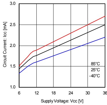
Fig.2 Supply current (2ch)
