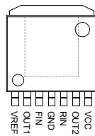
Fig.28 HRP7
