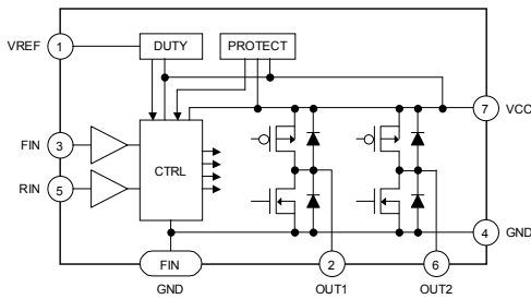
Fig.27 BD6210HFP / BD6211HFP / BD6212HFP
