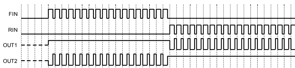
Fig.39 PWM control operation (timing chart)
