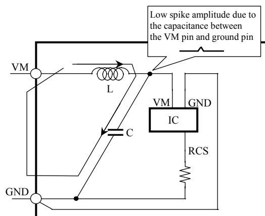
Fig. 5 Recommended PCB
